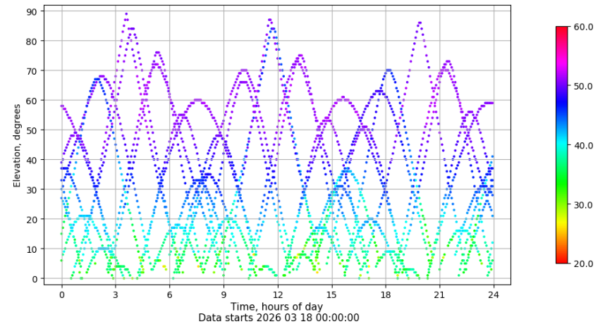
Time-elevation plot for station VIGO. Signal to Noise S1C Data file VIGO00ESP_R_2026077.xtr
