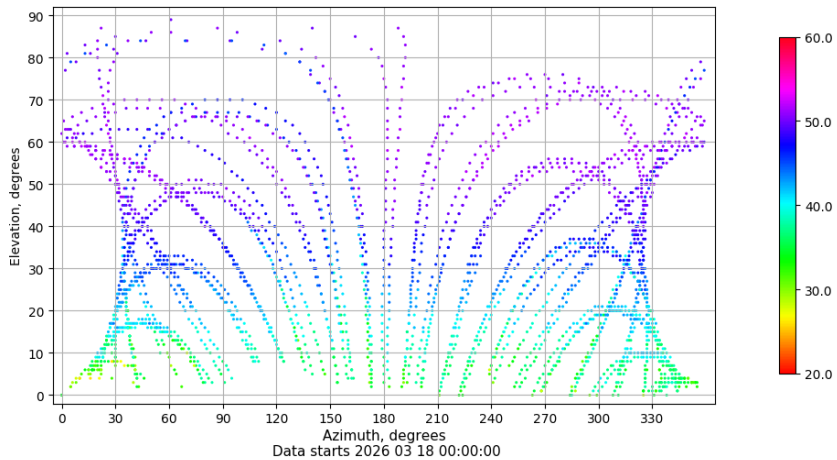
Azimuth-elevation plot for station VIGO. Signal to Noise S1C Data file VIGO00ESP_R_2026077.xtr
