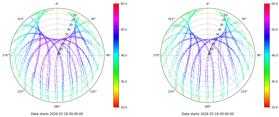
Skyplot for station VIGO. Signal to Noise S1C Data file VIGO00ESP_R_2026077.xtr Skyplot for station VIGO. Signal to Noise S2C Data file VIGO00ESP_R_2026077.xtr
