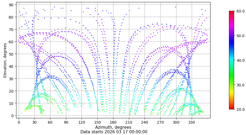
Azimuth-elevation plot for station VIGO. Signal to Noise S1C Data file VIGO00ESP_R_2026076.xtr
