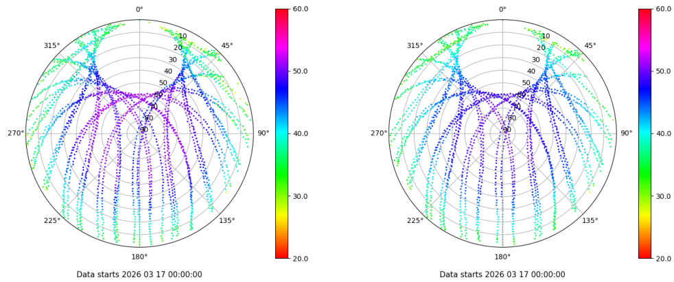
Skyplot for station VIGO. Signal to Noise S1C Data file VIGO00ESP_R_2026076.xtr Skyplot for station VIGO. Signal to Noise S2C Data file VIGO00ESP_R_2026076.xtr
