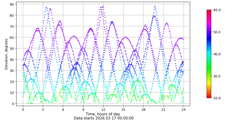
Time-elevation plot for station VIGO. Signal to Noise S1C Data file VIGO00ESP_R_2026076.xtr
