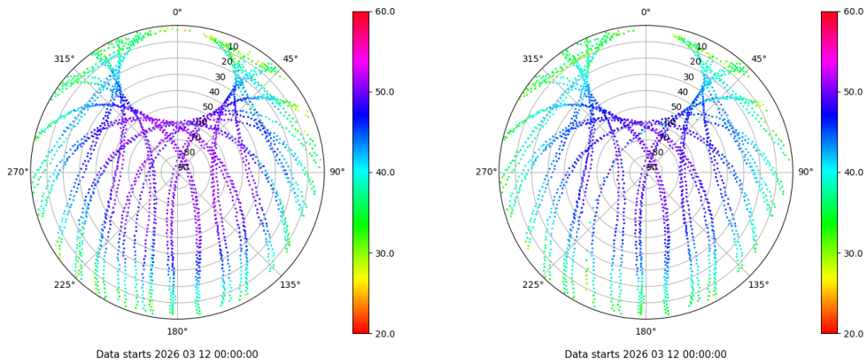
Skyplot for station VIGO. Signal to Noise S1C Data file VIGO00ESP_R_2026071.xtr Skyplot for station VIGO. Signal to Noise S2C Data file VIGO00ESP_R_2026071.xtr
