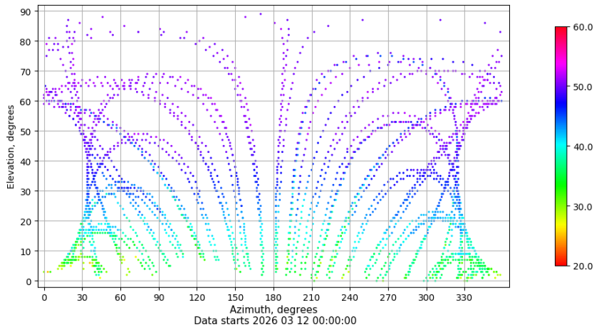
Azimuth-elevation plot for station VIGO. Signal to Noise S1C Data file VIGO00ESP_R_2026071.xtr
