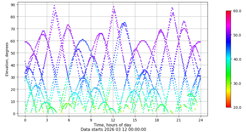
Time-elevation plot for station VIGO. Signal to Noise S1C Data file VIGO00ESP_R_2026071.xtr
