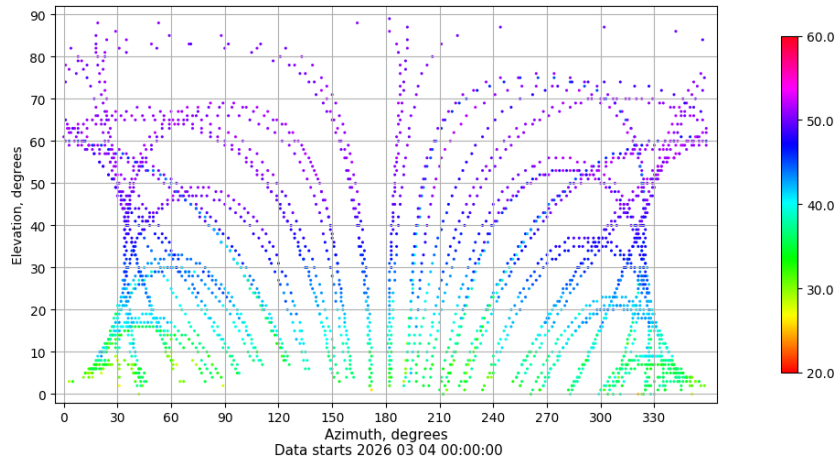
Azimuth-elevation plot for station VIGO. Signal to Noise S1C Data file VIGO00ESP_R_2026063.xtr
