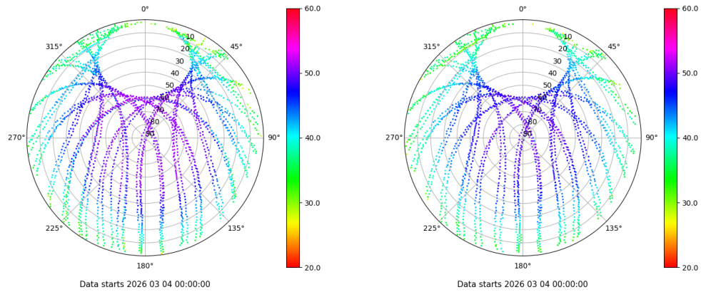
Skyplot for station VIGO. Signal to Noise S1C Data file VIGO00ESP_R_2026063.xtr Skyplot for station VIGO. Signal to Noise S2C Data file VIGO00ESP_R_2026063.xtr
