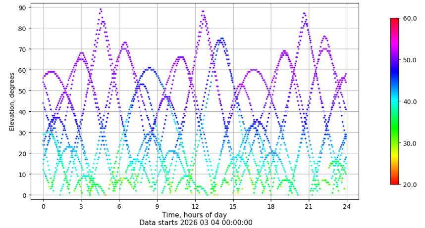
Time-elevation plot for station VIGO. Signal to Noise S1C Data file VIGO00ESP_R_2026063.xtr
