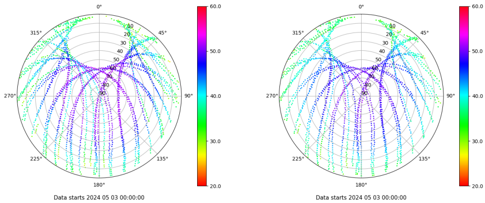
Skyplot for station VIGO. Signal to Noise S1C Data file VIGO00ESP_R_2024124.xtr Skyplot for station VIGO. Signal to Noise S2C Data file VIGO00ESP_R_2024124.xtr
