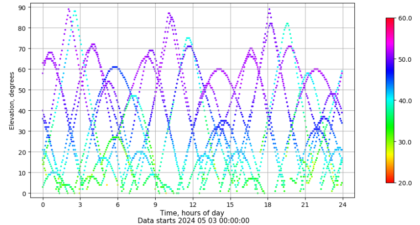
Time-elevation plot for station VIGO. Signal to Noise S1C Data file VIGO00ESP_R_2024124.xtr
