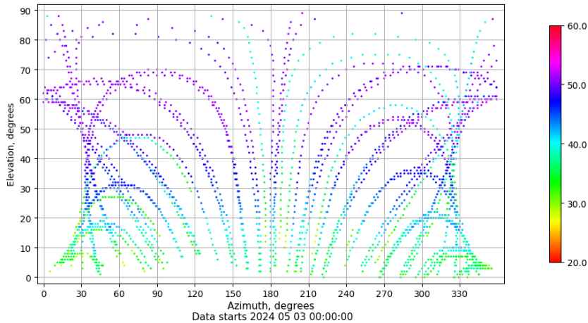
Azimuth-elevation plot for station VIGO. Signal to Noise S1C Data file VIGO00ESP_R_2024124.xtr
