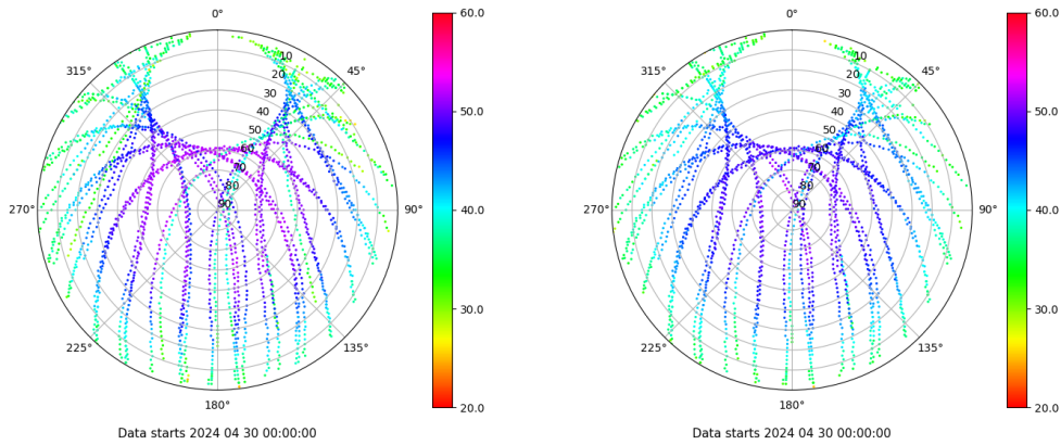
Skyplot for station VIGO. Signal to Noise S1C Data file VIGO00ESP_R_2024121.xtr Skyplot for station VIGO. Signal to Noise S2C Data file VIGO00ESP_R_2024121.xtr
