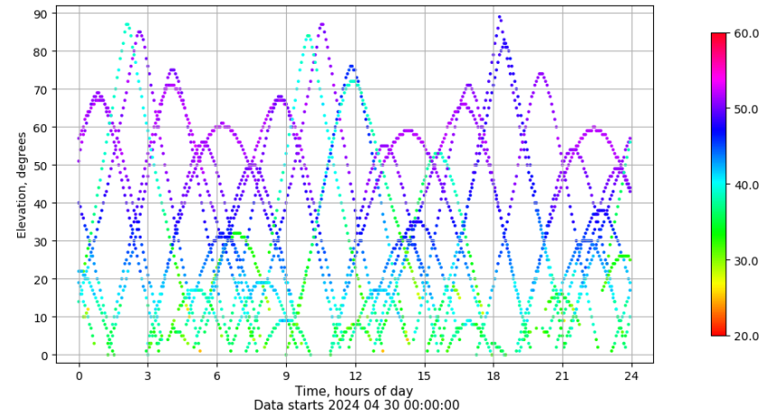
Time-elevation plot for station VIGO. Signal to Noise S1C Data file VIGO00ESP_R_2024121.xtr
