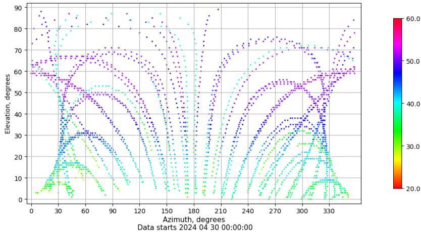
Azimuth-elevation plot for station VIGO. Signal to Noise S1C Data file VIGO00ESP_R_2024121.xtr
