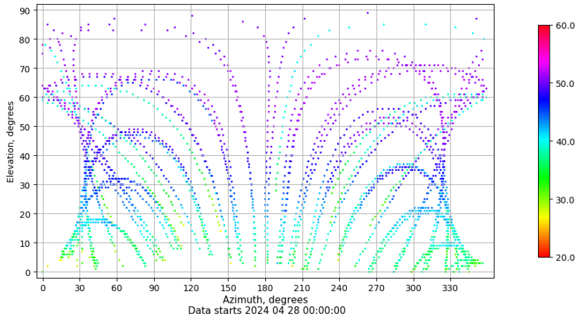
Azimuth-elevation plot for station VIGO. Signal to Noise S1C Data file VIGO00ESP_R_2024119.xtr
