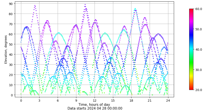
Time-elevation plot for station VIGO. Signal to Noise S1C Data file VIGO00ESP_R_2024119.xtr
