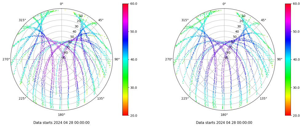
Skyplot for station VIGO. Signal to Noise S1C Data file VIGO00ESP_R_2024119.xtr Skyplot for station VIGO. Signal to Noise S2C Data file VIGO00ESP_R_2024119.xtr
