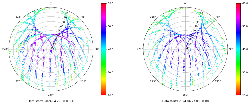
Skyplot for station VIGO. Signal to Noise S1C Data file VIGO00ESP_R_2024118.xtr Skyplot for station VIGO. Signal to Noise S2C Data file VIGO00ESP_R_2024118.xtr
