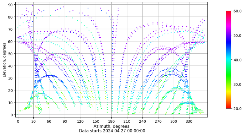
Azimuth-elevation plot for station VIGO. Signal to Noise S1C Data file VIGO00ESP_R_2024118.xtr
