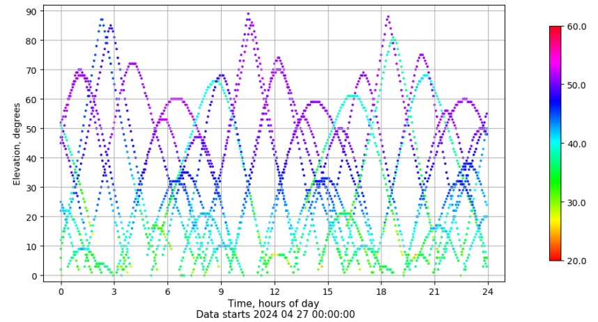
Time-elevation plot for station VIGO. Signal to Noise S1C Data file VIGO00ESP_R_2024118.xtr
