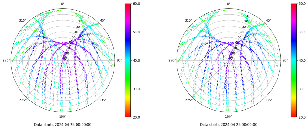
Skyplot for station VIGO. Signal to Noise S1C Data file VIGO00ESP_R_2024116.xtr Skyplot for station VIGO. Signal to Noise S2C Data file VIGO00ESP_R_2024116.xtr
