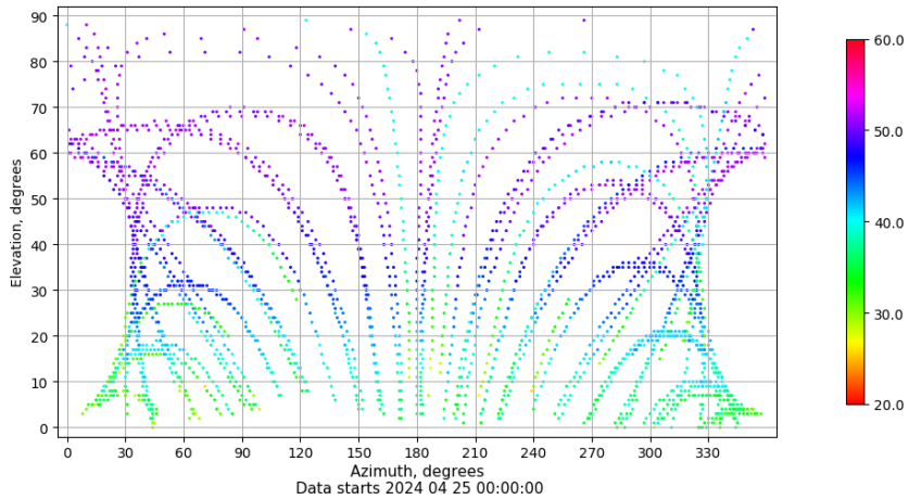
Azimuth-elevation plot for station VIGO. Signal to Noise S1C Data file VIGO00ESP_R_2024116.xtr
