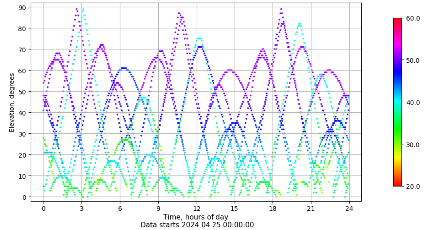
Time-elevation plot for station VIGO. Signal to Noise S1C Data file VIGO00ESP_R_2024116.xtr
