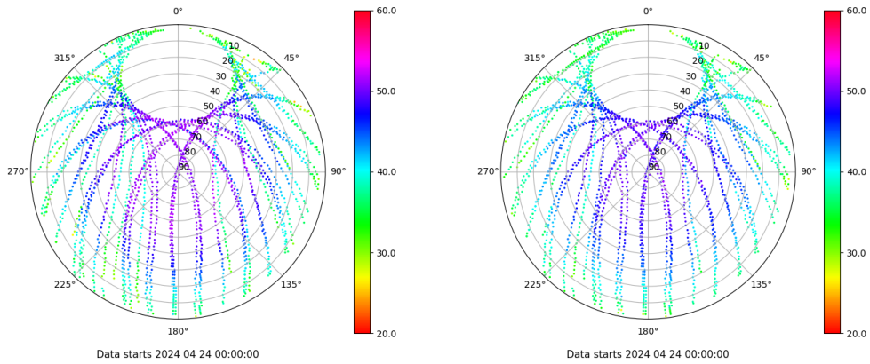
Skyplot for station VIGO. Signal to Noise S1C Data file VIGO00ESP_R_2024115.xtr Skyplot for station VIGO. Signal to Noise S2C Data file VIGO00ESP_R_2024115.xtr
