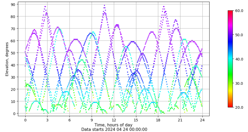
Time-elevation plot for station VIGO. Signal to Noise S1C Data file VIGO00ESP_R_2024115.xtr
