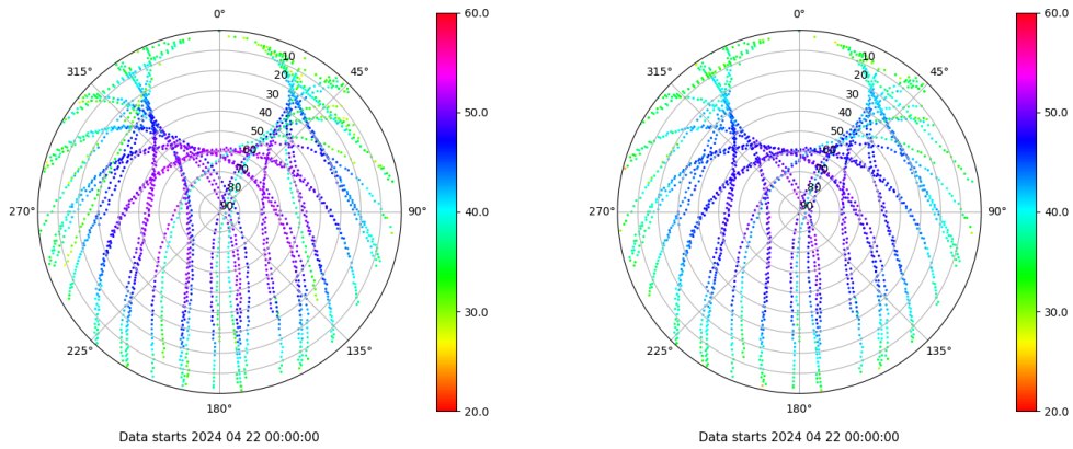
Skyplot for station VIGO. Signal to Noise S1C Data file VIGO00ESP_R_2024113.xtr Skyplot for station VIGO. Signal to Noise S2C Data file VIGO00ESP_R_2024113.xtr
