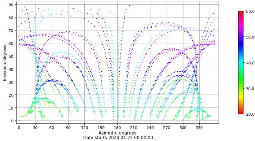
Azimuth-elevation plot for station VIGO. Signal to Noise S1C Data file VIGO00ESP_R_2024113.xtr
