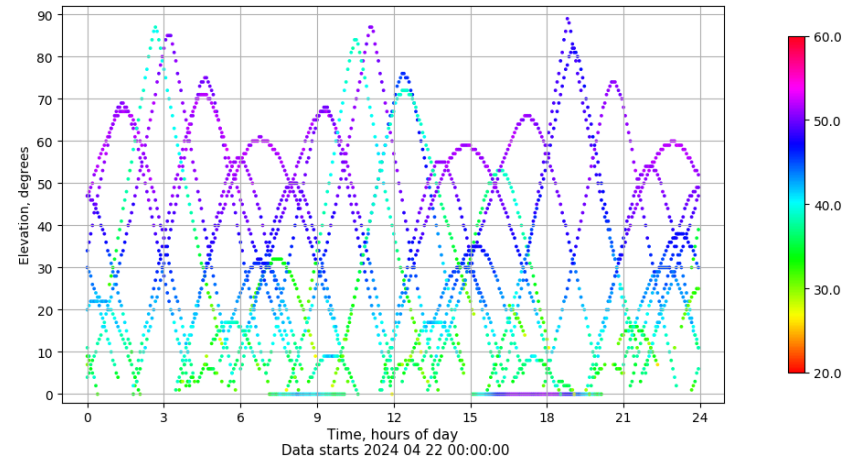
Time-elevation plot for station VIGO. Signal to Noise S1C Data file VIGO00ESP_R_2024113.xtr
