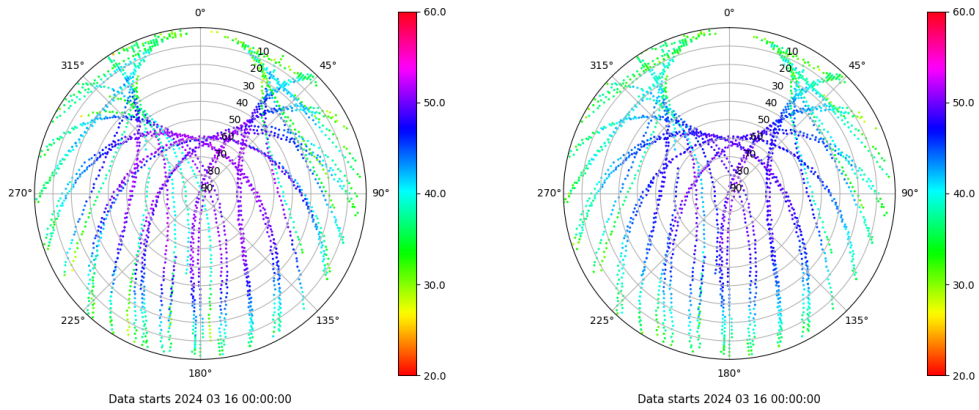
Skyplot for station VIGO. Signal to Noise S1C Data file VIGO00ESP_R_2024076.xtr Skyplot for station VIGO. Signal to Noise S2C Data file VIGO00ESP_R_2024076.xtr
