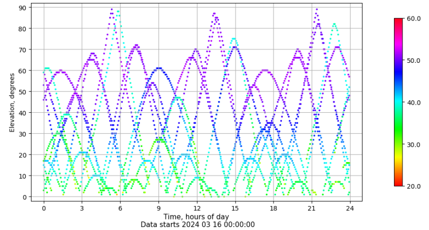
Time-elevation plot for station VIGO. Signal to Noise S1C Data file VIGO00ESP_R_2024076.xtr
