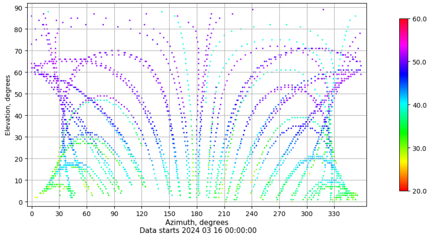
Azimuth-elevation plot for station VIGO. Signal to Noise S1C Data file VIGO00ESP_R_2024076.xtr
