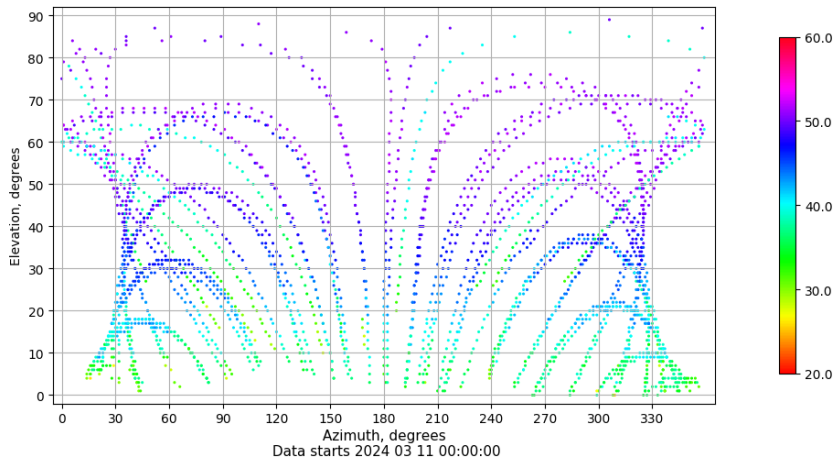
Azimuth-elevation plot for station VIGO. Signal to Noise S1C Data file VIGO00ESP_R_2024071.xtr
