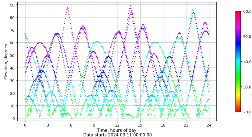
Time-elevation plot for station VIGO. Signal to Noise S1C Data file VIGO00ESP_R_2024071.xtr
