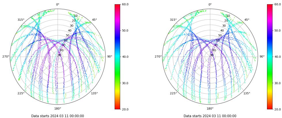
Skyplot for station VIGO. Signal to Noise S1C Data file VIGO00ESP_R_2024071.xtr Skyplot for station VIGO. Signal to Noise S2C Data file VIGO00ESP_R_2024071.xtr
