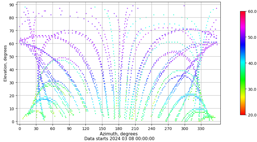
Azimuth-elevation plot for station VIGO. Signal to Noise S1C Data file VIGO00ESP_R_2024068.xtr
