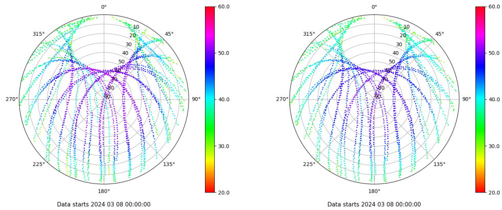
Skyplot for station VIGO. Signal to Noise S1C Data file VIGO00ESP_R_2024068.xtr Skyplot for station VIGO. Signal to Noise S2C Data file VIGO00ESP_R_2024068.xtr
