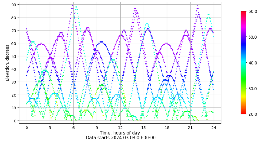
Time-elevation plot for station VIGO. Signal to Noise S1C Data file VIGO00ESP_R_2024068.xtr
