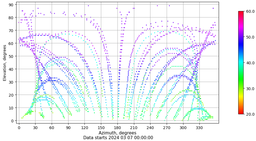
Azimuth-elevation plot for station VIGO. Signal to Noise S1C Data file VIGO00ESP_R_2024067.xtr
