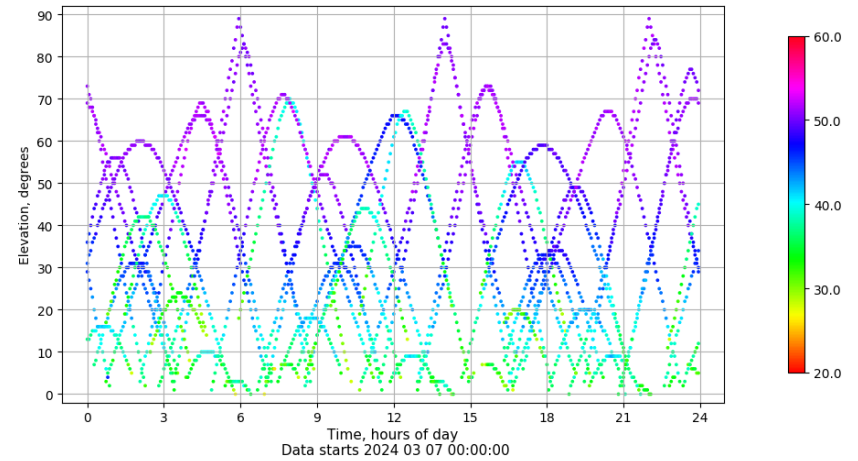
Time-elevation plot for station VIGO. Signal to Noise S1C Data file VIGO00ESP_R_2024067.xtr
