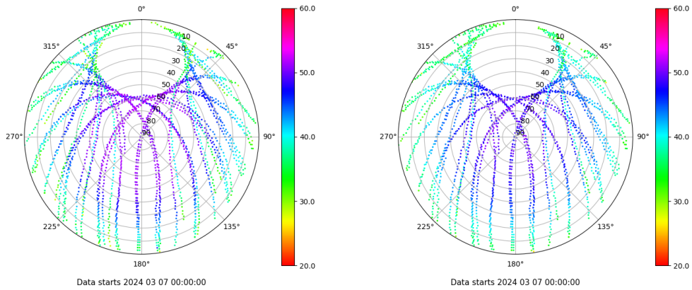
Skyplot for station VIGO. Signal to Noise S1C Data file VIGO00ESP_R_2024067.xtr Skyplot for station VIGO. Signal to Noise S2C Data file VIGO00ESP_R_2024067.xtr
