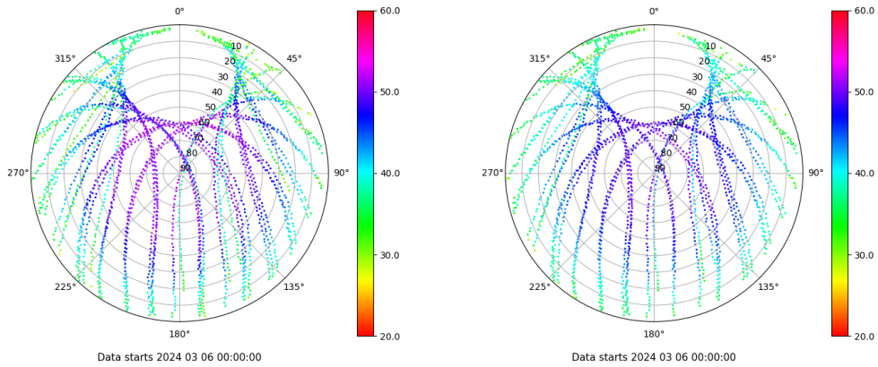
Skyplot for station VIGO. Signal to Noise S1C Data file VIGO00ESP_R_2024066.xtr Skyplot for station VIGO. Signal to Noise S2C Data file VIGO00ESP_R_2024066.xtr
