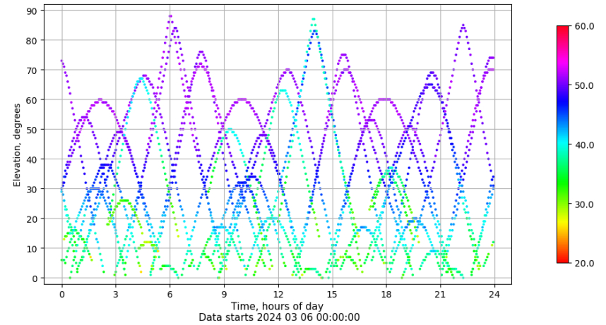
Time-elevation plot for station VIGO. Signal to Noise S1C Data file VIGO00ESP_R_2024066.xtr
