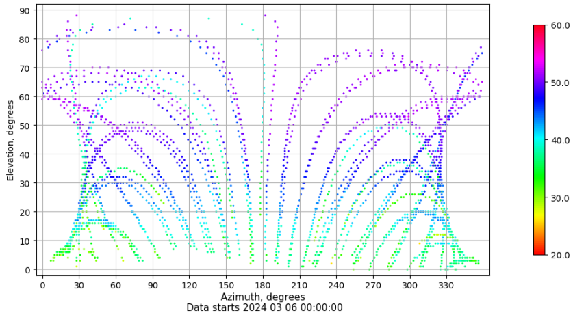
Azimuth-elevation plot for station VIGO. Signal to Noise S1C Data file VIGO00ESP_R_2024066.xtr
