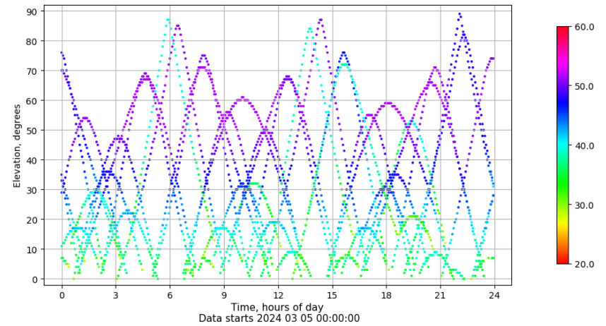
Time-elevation plot for station VIGO. Signal to Noise S1C Data file VIGO00ESP_R_2024065.xtr
