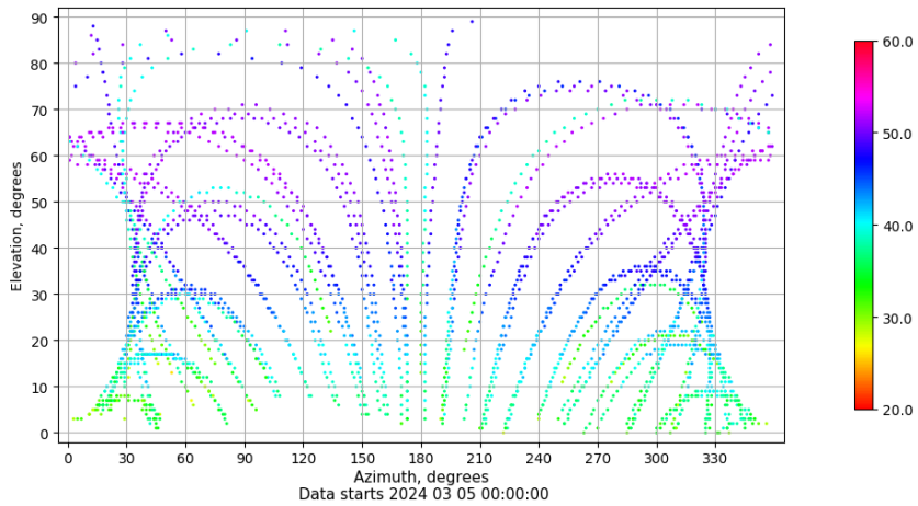
Azimuth-elevation plot for station VIGO. Signal to Noise S1C Data file VIGO00ESP_R_2024065.xtr
