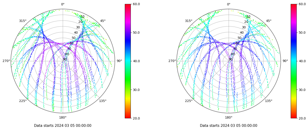
Skyplot for station VIGO. Signal to Noise S1C Data file VIGO00ESP_R_2024065.xtr Skyplot for station VIGO. Signal to Noise S2C Data file VIGO00ESP_R_2024065.xtr
