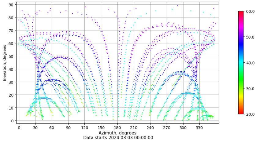
Azimuth-elevation plot for station VIGO. Signal to Noise S1C Data file VIGO00ESP_R_2024063.xtr
