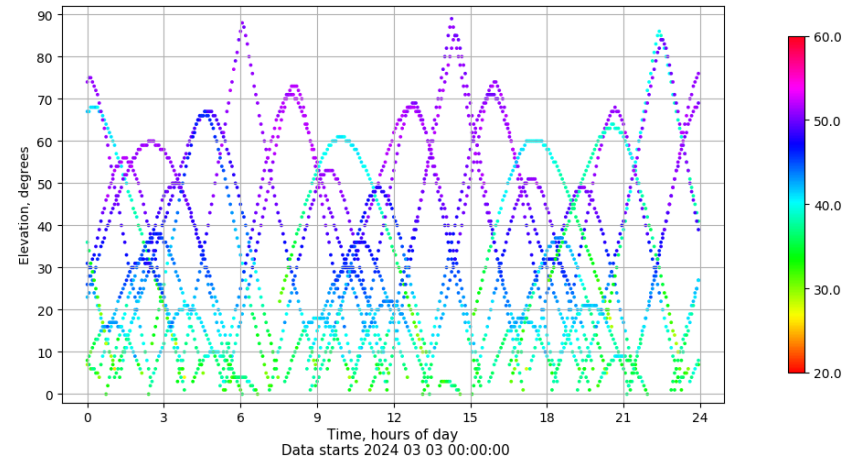
Time-elevation plot for station VIGO. Signal to Noise S1C Data file VIGO00ESP_R_2024063.xtr
