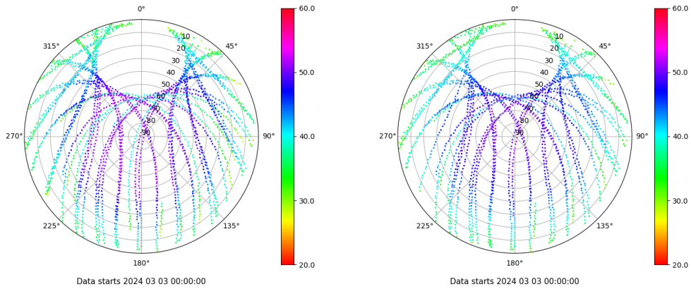
Skyplot for station VIGO. Signal to Noise S1C Data file VIGO00ESP_R_2024063.xtr Skyplot for station VIGO. Signal to Noise S2C Data file VIGO00ESP_R_2024063.xtr
