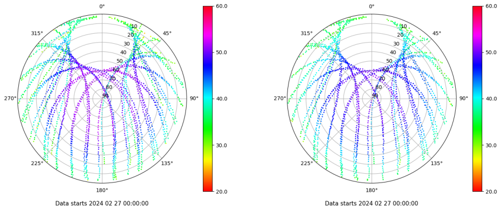
Skyplot for station VIGO. Signal to Noise S1C Data file VIGO00ESP_R_2024058.xtr Skyplot for station VIGO. Signal to Noise S2C Data file VIGO00ESP_R_2024058.xtr
