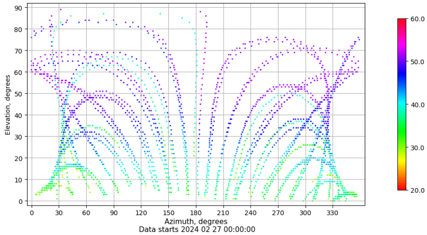
Azimuth-elevation plot for station VIGO. Signal to Noise S1C Data file VIGO00ESP_R_2024058.xtr
