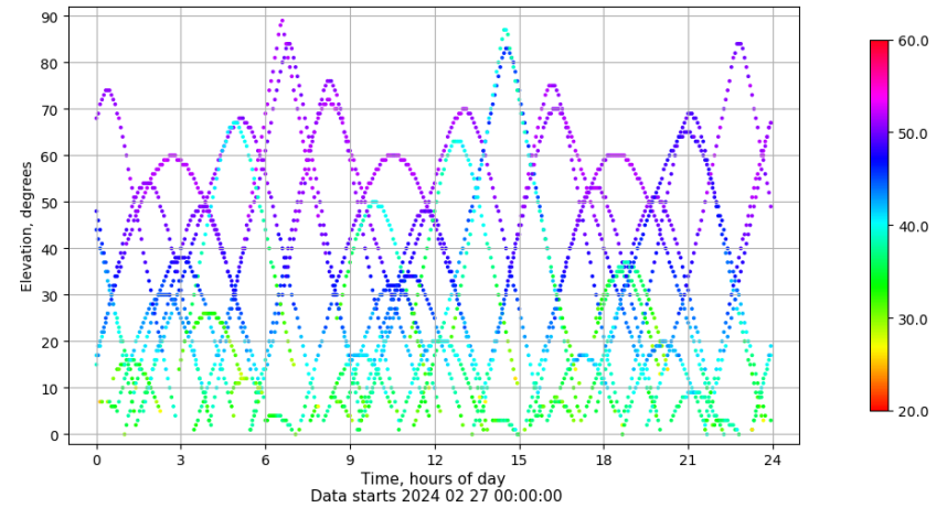
Time-elevation plot for station VIGO. Signal to Noise S1C Data file VIGO00ESP_R_2024058.xtr
