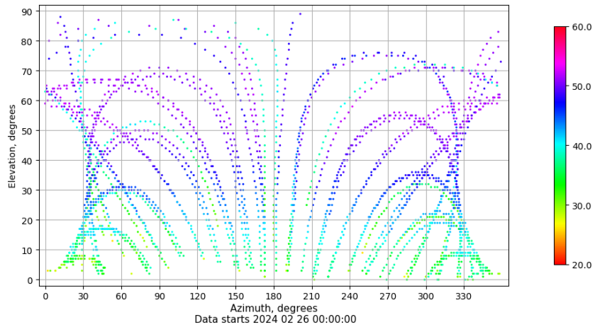
Azimuth-elevation plot for station VIGO. Signal to Noise S1C Data file VIGO00ESP_R_2024057.xtr
