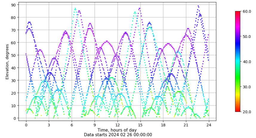
Time-elevation plot for station VIGO. Signal to Noise S1C Data file VIGO00ESP_R_2024057.xtr
