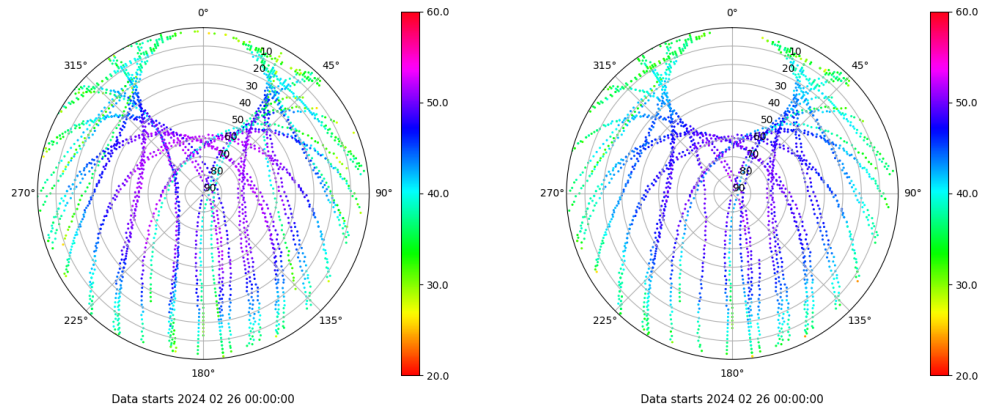
Skyplot for station VIGO. Signal to Noise S1C Data file VIGO00ESP_R_2024057.xtr Skyplot for station VIGO. Signal to Noise S2C Data file VIGO00ESP_R_2024057.xtr
