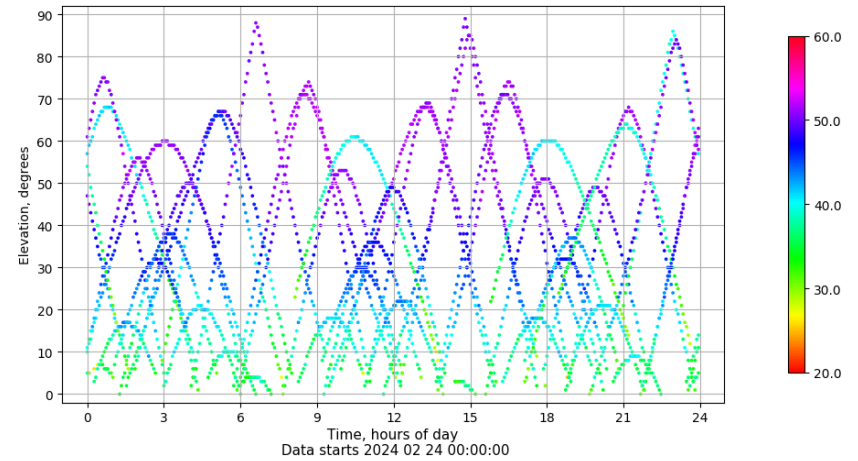
Time-elevation plot for station VIGO. Signal to Noise S1C Data file VIGO00ESP_R_2024055.xtr
