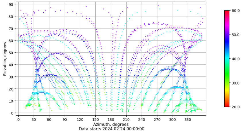
Azimuth-elevation plot for station VIGO. Signal to Noise S1C Data file VIGO00ESP_R_2024055.xtr
