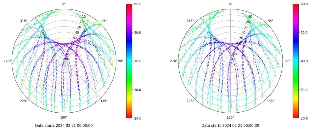
Skyplot for station VIGO. Signal to Noise S1C Data file VIGO00ESP_R_2024052.xtr Skyplot for station VIGO. Signal to Noise S2C Data file VIGO00ESP_R_2024052.xtr
