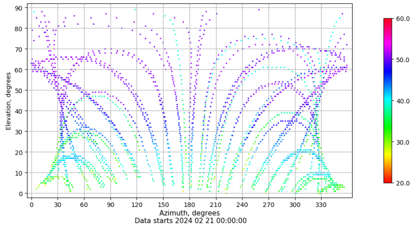
Azimuth-elevation plot for station VIGO. Signal to Noise S1C Data file VIGO00ESP_R_2024052.xtr
