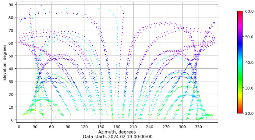
Azimuth-elevation plot for station VIGO. Signal to Noise S1C Data file VIGO00ESP_R_2024050.xtr
