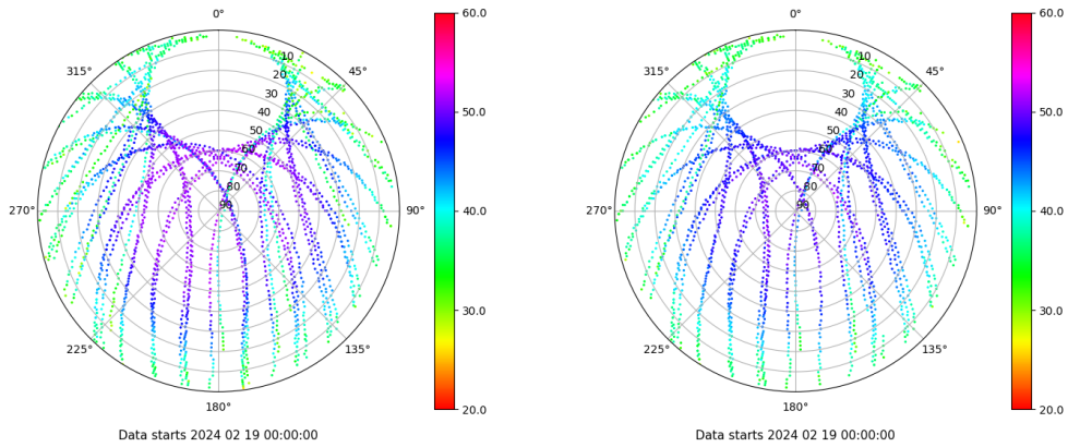
Skyplot for station VIGO. Signal to Noise S1C Data file VIGO00ESP_R_2024050.xtr Skyplot for station VIGO. Signal to Noise S2C Data file VIGO00ESP_R_2024050.xtr
