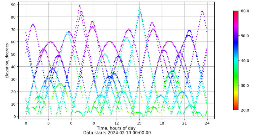
Time-elevation plot for station VIGO. Signal to Noise S1C Data file VIGO00ESP_R_2024050.xtr
