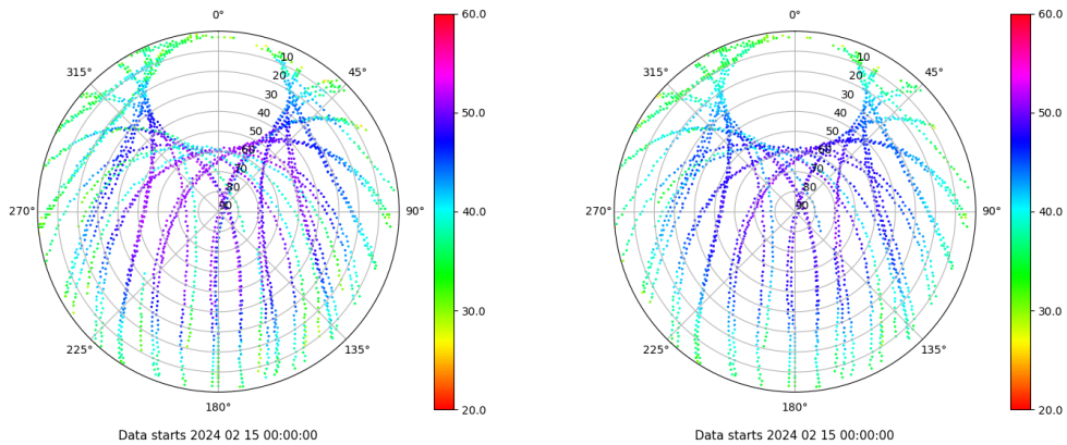
Skyplot for station VIGO. Signal to Noise S1C Data file VIGO00ESP_R_2024046.xtr Skyplot for station VIGO. Signal to Noise S2C Data file VIGO00ESP_R_2024046.xtr
