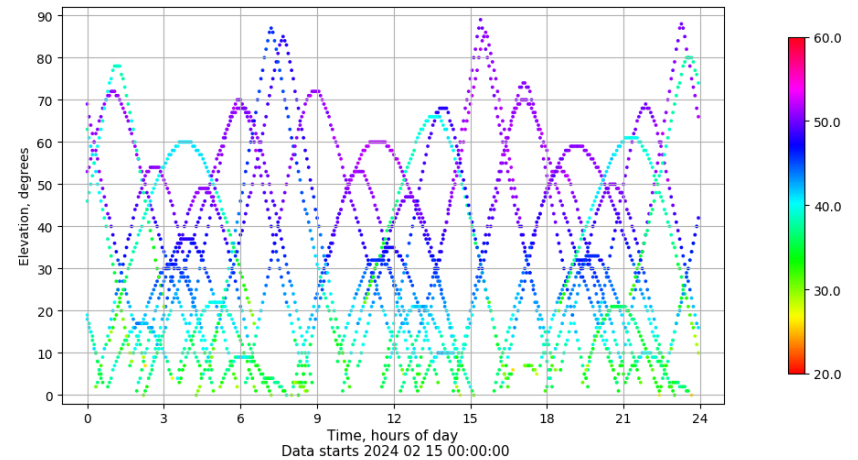
Time-elevation plot for station VIGO. Signal to Noise S1C Data file VIGO00ESP_R_2024046.xtr
