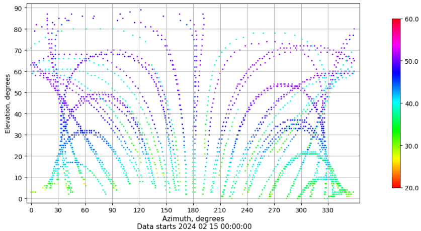
Azimuth-elevation plot for station VIGO. Signal to Noise S1C Data file VIGO00ESP_R_2024046.xtr
