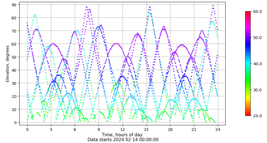
Time-elevation plot for station VIGO. Signal to Noise S1C Data file VIGO00ESP_R_2024045.xtr
