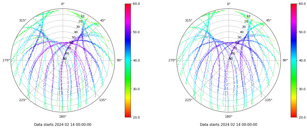
Skyplot for station VIGO. Signal to Noise S1C Data file VIGO00ESP_R_2024045.xtr Skyplot for station VIGO. Signal to Noise S2C Data file VIGO00ESP_R_2024045.xtr
