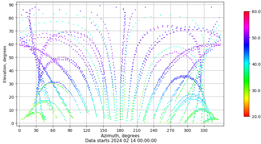
Azimuth-elevation plot for station VIGO. Signal to Noise S1C Data file VIGO00ESP_R_2024045.xtr
