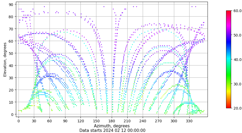
Azimuth-elevation plot for station VIGO. Signal to Noise S1C Data file VIGO00ESP_R_2024043.xtr
