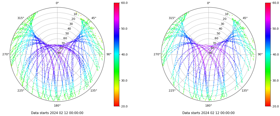
Skyplot for station VIGO. Signal to Noise S1C Data file VIGO00ESP_R_2024043.xtr Skyplot for station VIGO. Signal to Noise S2X Data file VIGO00ESP_R_2024043.xtr
