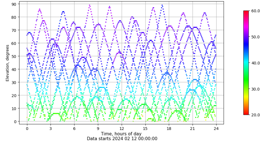
Time-elevation plot for station VIGO. Signal to Noise S1C Data file VIGO00ESP_R_2024043.xtr
