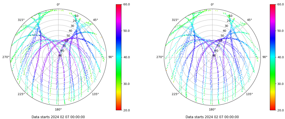
Skyplot for station VIGO. Signal to Noise S1C Data file VIGO00ESP_R_2024038.xtr Skyplot for station VIGO. Signal to Noise S2C Data file VIGO00ESP_R_2024038.xtr
