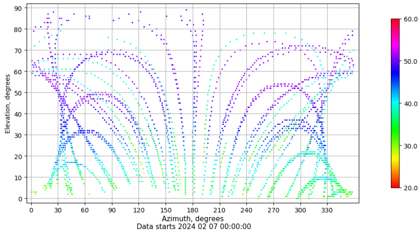
Azimuth-elevation plot for station VIGO. Signal to Noise S1C Data file VIGO00ESP_R_2024038.xtr
