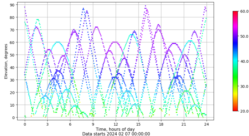
Time-elevation plot for station VIGO. Signal to Noise S1C Data file VIGO00ESP_R_2024038.xtr
