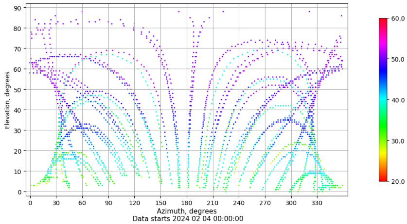
Azimuth-elevation plot for station VIGO. Signal to Noise S1C Data file VIGO00ESP_R_2024035.xtr
