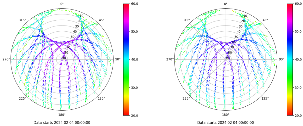
Skyplot for station VIGO. Signal to Noise S1C Data file VIGO00ESP_R_2024035.xtr Skyplot for station VIGO. Signal to Noise S2C Data file VIGO00ESP_R_2024035.xtr
