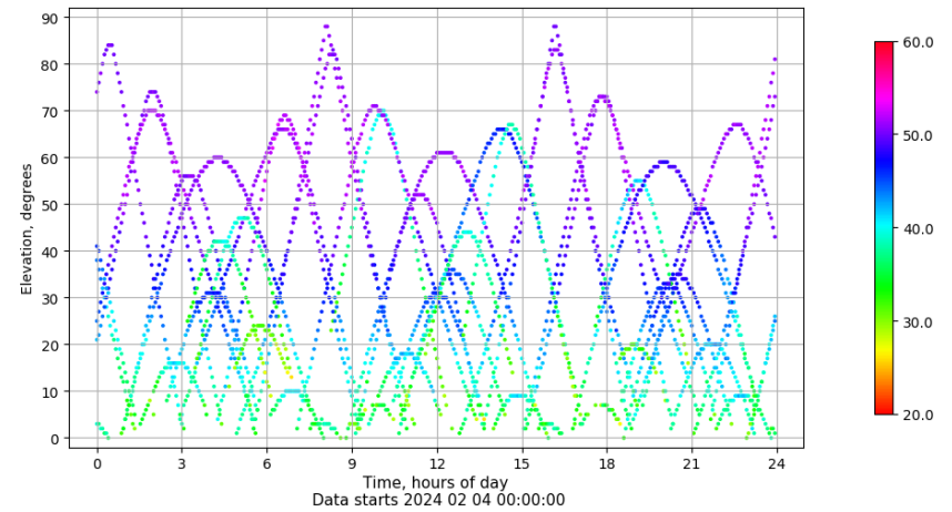
Time-elevation plot for station VIGO. Signal to Noise S1C Data file VIGO00ESP_R_2024035.xtr
