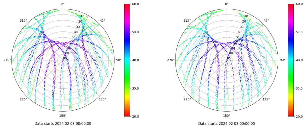
Skyplot for station VIGO. Signal to Noise S1C Data file VIGO00ESP_R_2024034.xtr Skyplot for station VIGO. Signal to Noise S2C Data file VIGO00ESP_R_2024034.xtr
