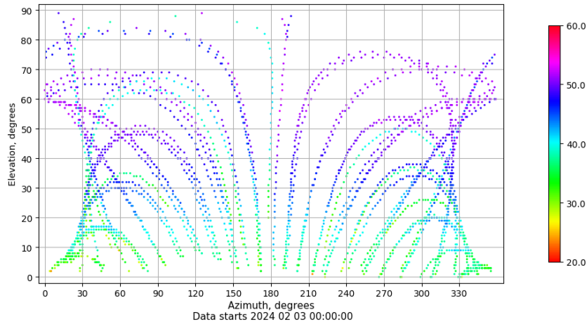
Azimuth-elevation plot for station VIGO. Signal to Noise S1C Data file VIGO00ESP_R_2024034.xtr
