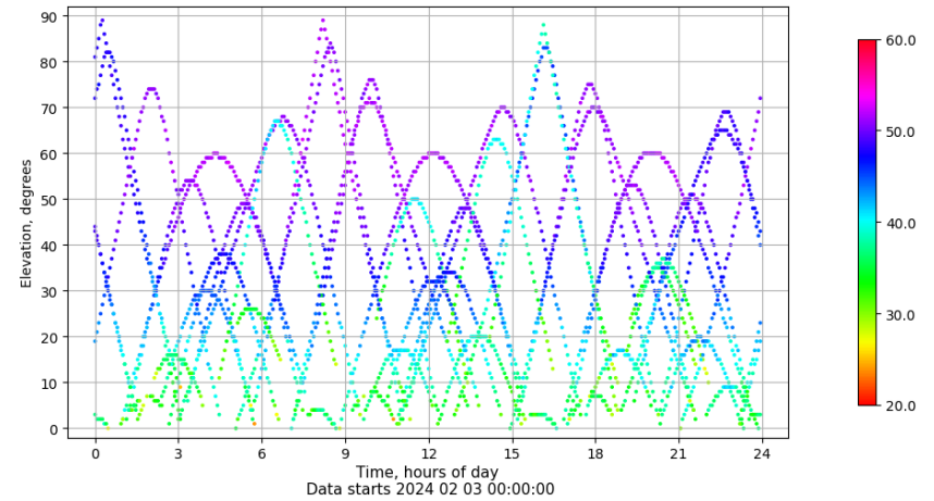
Time-elevation plot for station VIGO. Signal to Noise S1C Data file VIGO00ESP_R_2024034.xtr
