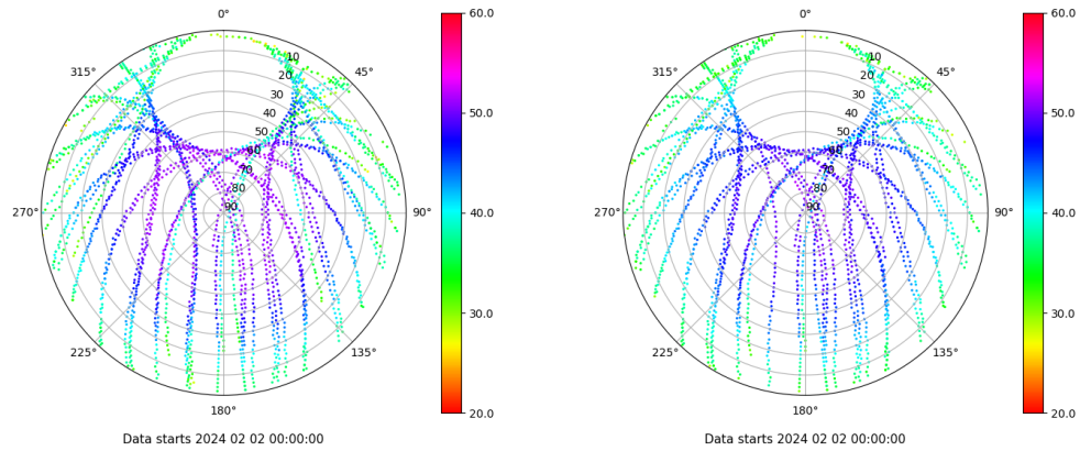
Skyplot for station VIGO. Signal to Noise S1C Data file VIGO00ESP_R_2024033.xtr Skyplot for station VIGO. Signal to Noise S2C Data file VIGO00ESP_R_2024033.xtr
