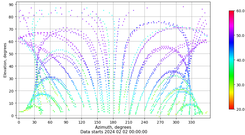
Azimuth-elevation plot for station VIGO. Signal to Noise S1C Data file VIGO00ESP_R_2024033.xtr
