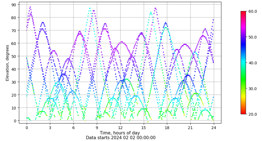
Time-elevation plot for station VIGO. Signal to Noise S1C Data file VIGO00ESP_R_2024033.xtr
