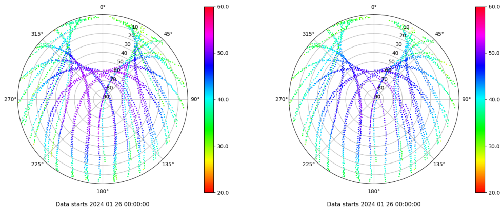
Skyplot for station VIGO. Signal to Noise S1C Data file VIGO00ESP_R_2024026.xtr Skyplot for station VIGO. Signal to Noise S2C Data file VIGO00ESP_R_2024026.xtr
