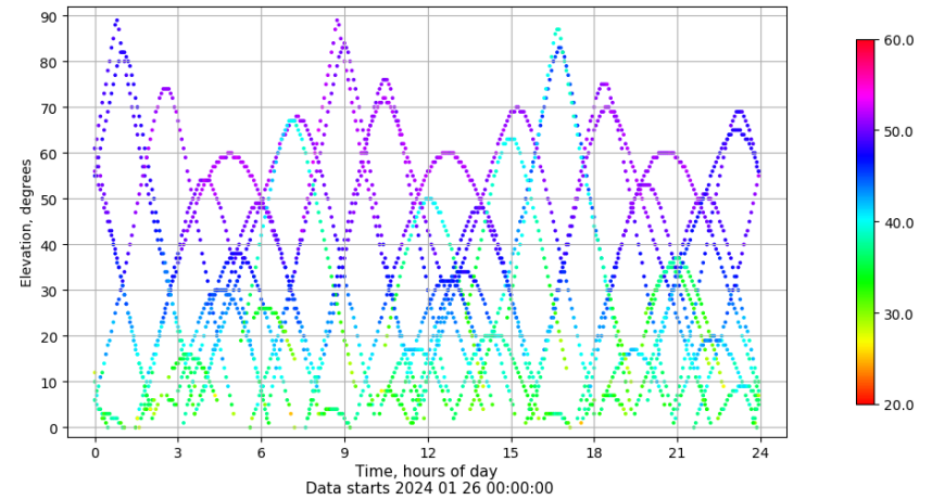
Time-elevation plot for station VIGO. Signal to Noise S1C Data file VIGO00ESP_R_2024026.xtr
