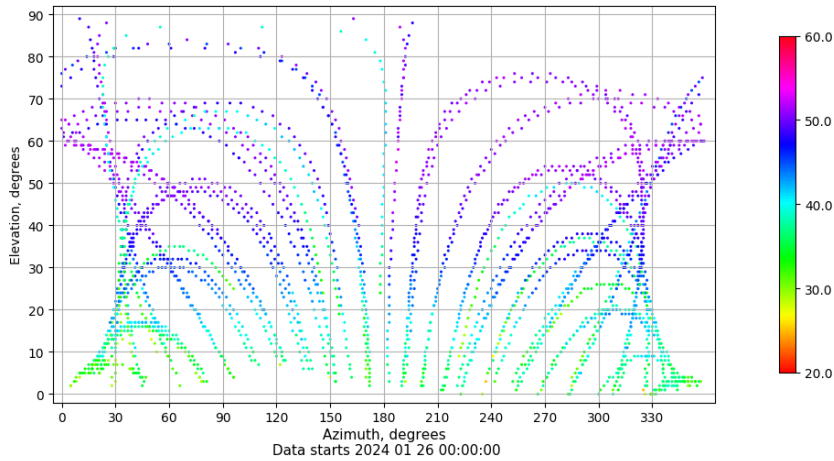
Azimuth-elevation plot for station VIGO. Signal to Noise S1C Data file VIGO00ESP_R_2024026.xtr
