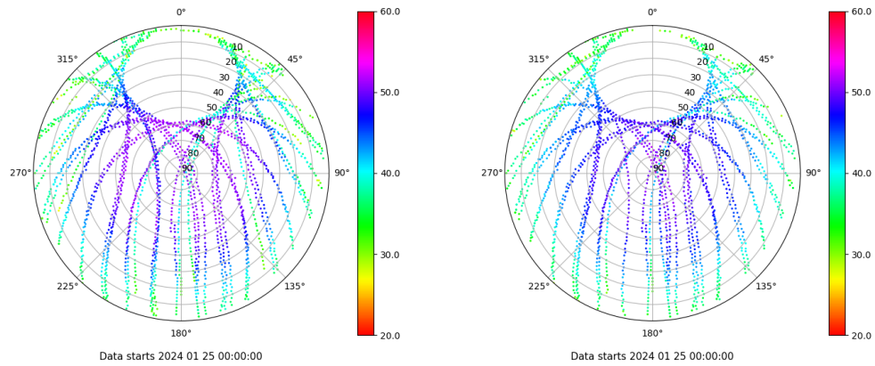
Skyplot for station VIGO. Signal to Noise S1C Data file VIGO00ESP_R_2024025.xtr Skyplot for station VIGO. Signal to Noise S2C Data file VIGO00ESP_R_2024025.xtr
