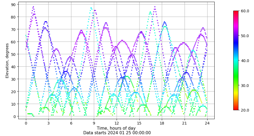
Time-elevation plot for station VIGO. Signal to Noise S1C Data file VIGO00ESP_R_2024025.xtr
