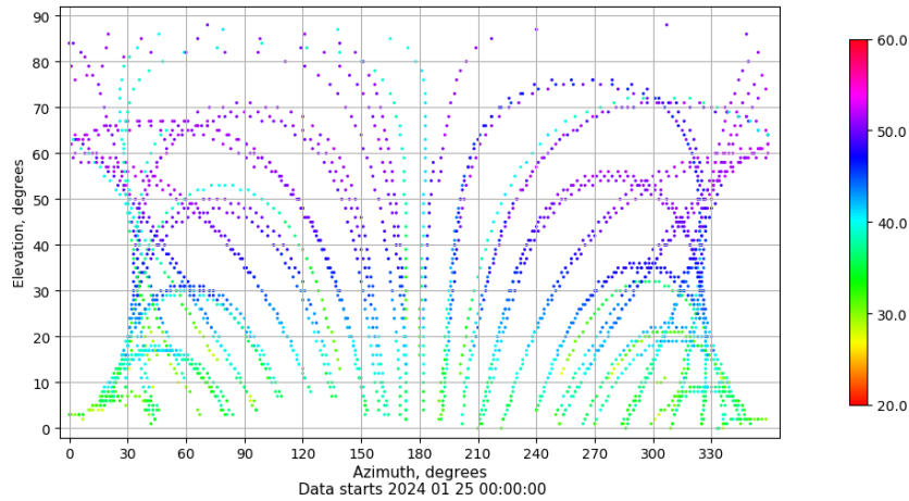
Azimuth-elevation plot for station VIGO. Signal to Noise S1C Data file VIGO00ESP_R_2024025.xtr
