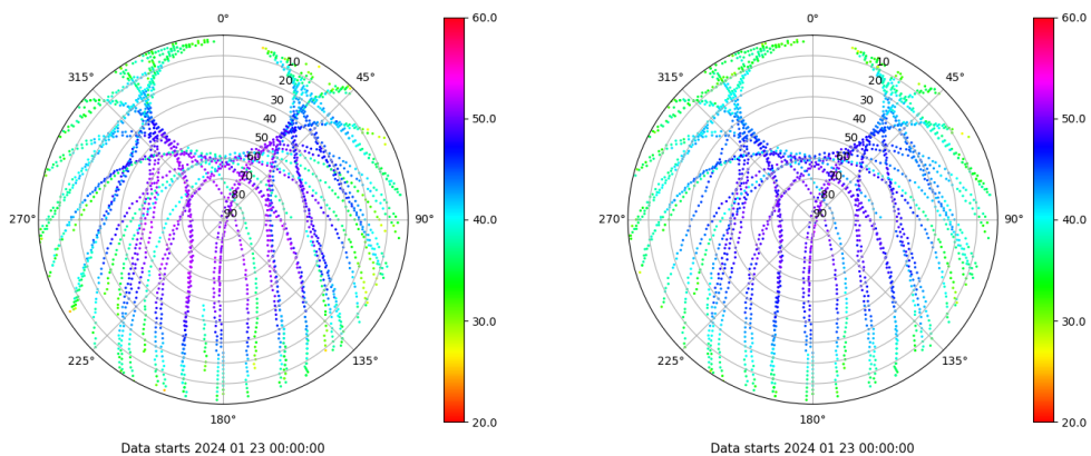
Skyplot for station VIGO. Signal to Noise S1C Data file VIGO00ESP_R_2024023.xtr Skyplot for station VIGO. Signal to Noise S2C Data file VIGO00ESP_R_2024023.xtr
