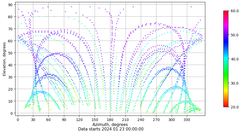
Azimuth-elevation plot for station VIGO. Signal to Noise S1C Data file VIGO00ESP_R_2024023.xtr
