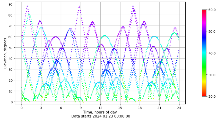
Time-elevation plot for station VIGO. Signal to Noise S1C Data file VIGO00ESP_R_2024023.xtr
