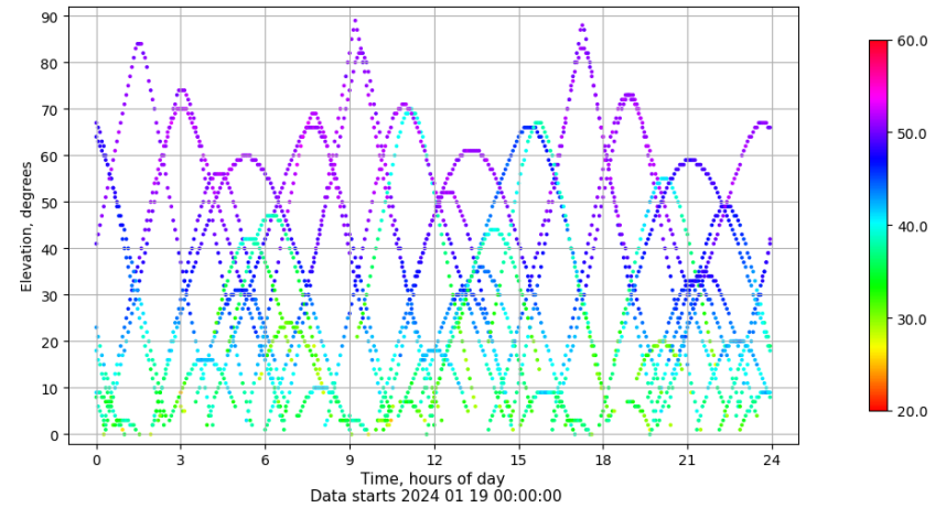
Time-elevation plot for station VIGO. Signal to Noise S1C Data file VIGO00ESP_R_2024019.xtr
