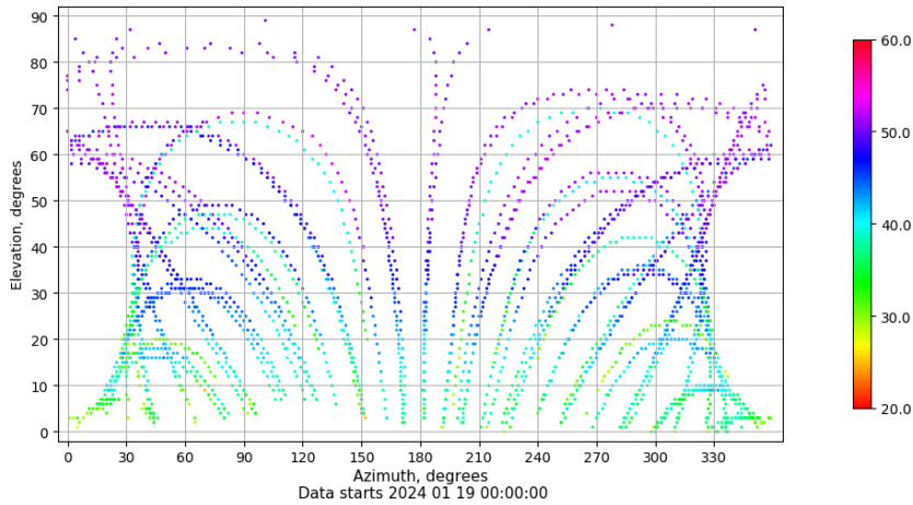
Azimuth-elevation plot for station VIGO. Signal to Noise S1C Data file VIGO00ESP_R_2024019.xtr
