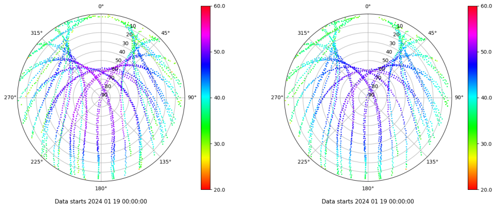
Skyplot for station VIGO. Signal to Noise S1C Data file VIGO00ESP_R_2024019.xtr Skyplot for station VIGO. Signal to Noise S2C Data file VIGO00ESP_R_2024019.xtr
