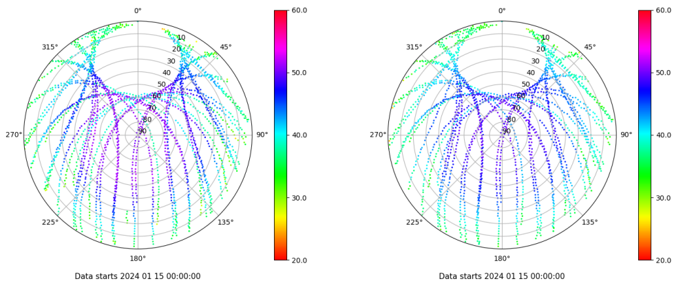
Skyplot for station VIGO. Signal to Noise S1C Data file VIGO00ESP_R_2024015.xtr Skyplot for station VIGO. Signal to Noise S2C Data file VIGO00ESP_R_2024015.xtr
