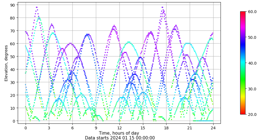
Time-elevation plot for station VIGO. Signal to Noise S1C Data file VIGO00ESP_R_2024015.xtr
