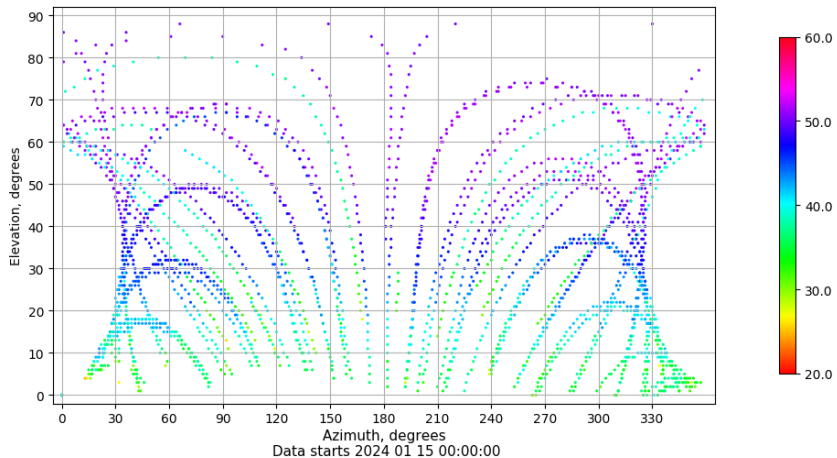
Azimuth-elevation plot for station VIGO. Signal to Noise S1C Data file VIGO00ESP_R_2024015.xtr
