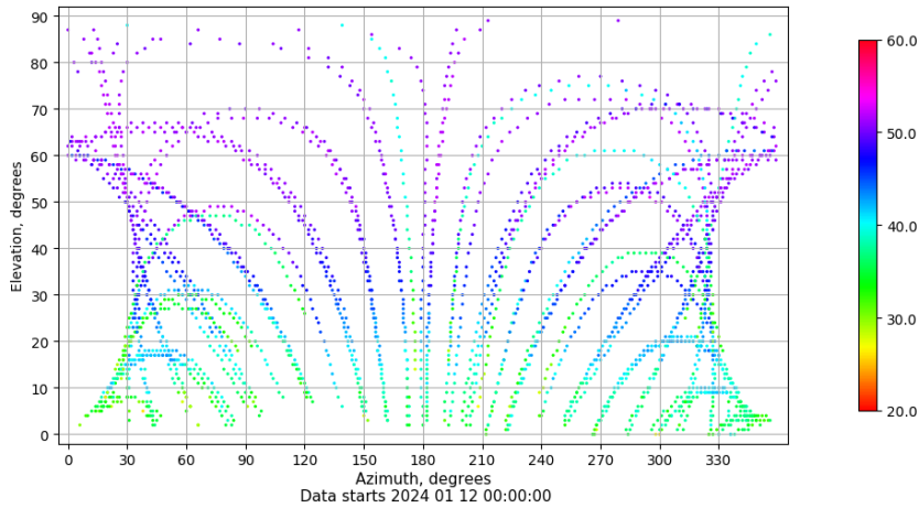
Azimuth-elevation plot for station VIGO. Signal to Noise S1C Data file VIGO00ESP_R_2024012.xtr
