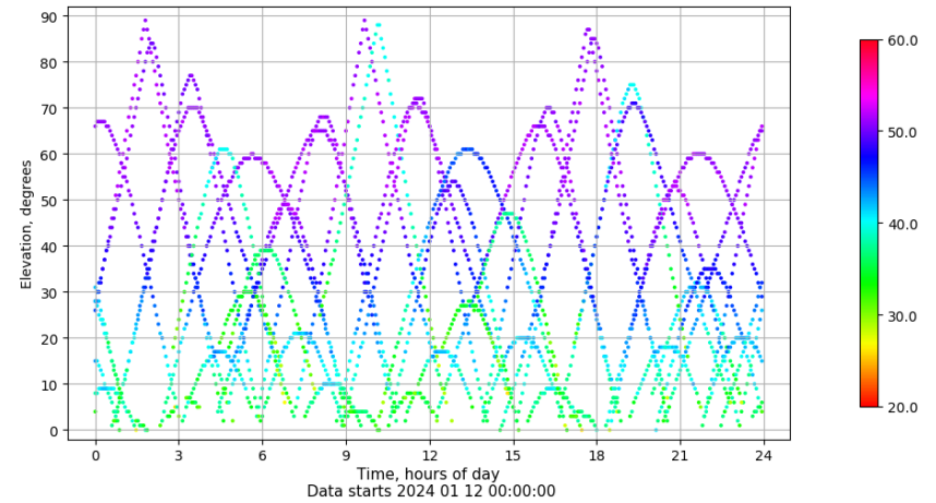
Time-elevation plot for station VIGO. Signal to Noise S1C Data file VIGO00ESP_R_2024012.xtr
