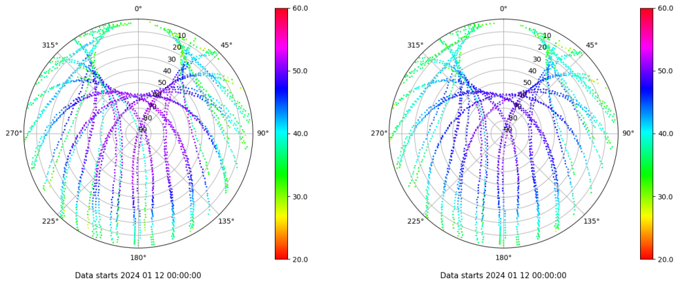
Skyplot for station VIGO. Signal to Noise S1C Data file VIGO00ESP_R_2024012.xtr Skyplot for station VIGO. Signal to Noise S2C Data file VIGO00ESP_R_2024012.xtr
