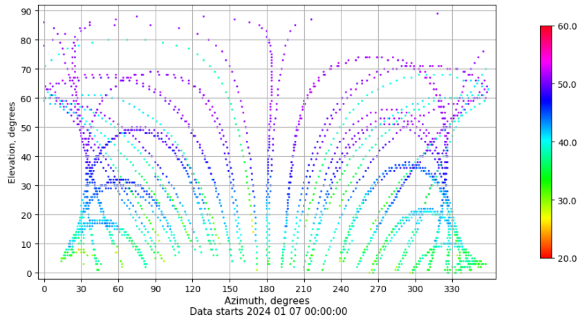
Azimuth-elevation plot for station VIGO. Signal to Noise S1C Data file VIGO00ESP_R_2024007.xtr
