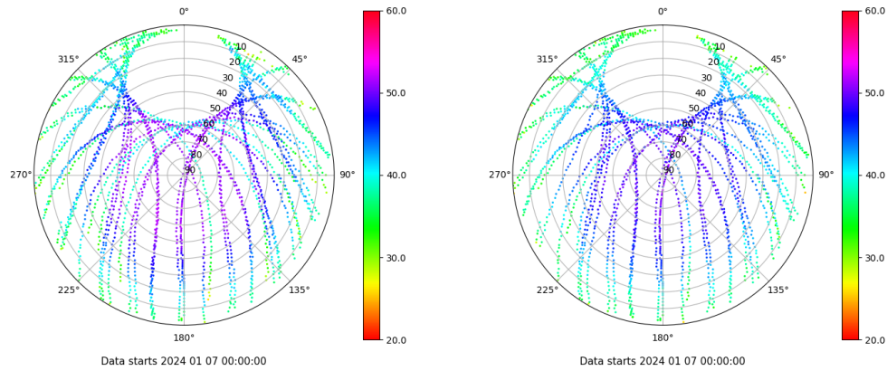
Skyplot for station VIGO. Signal to Noise S1C Data file VIGO00ESP_R_2024007.xtr Skyplot for station VIGO. Signal to Noise S2C Data file VIGO00ESP_R_2024007.xtr
