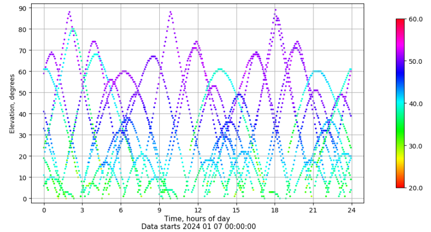
Time-elevation plot for station VIGO. Signal to Noise S1C Data file VIGO00ESP_R_2024007.xtr
