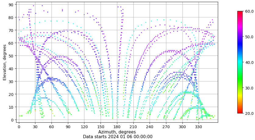
Azimuth-elevation plot for station VIGO. Signal to Noise S1C Data file VIGO00ESP_R_2024006.xtr
