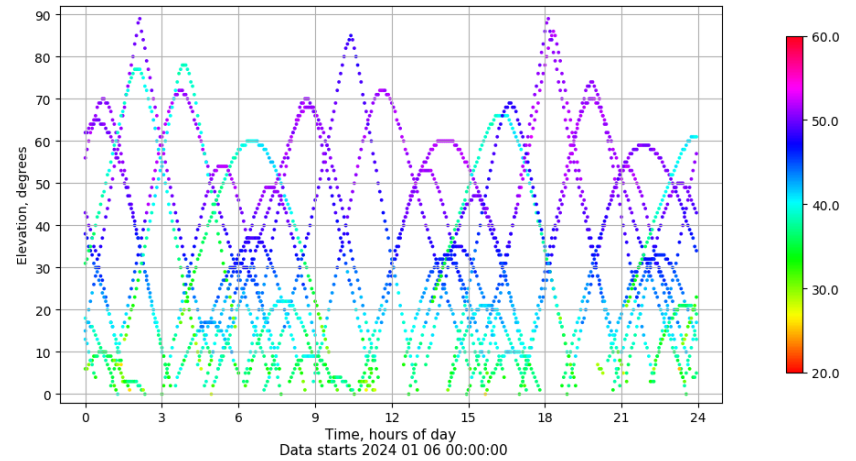
Time-elevation plot for station VIGO. Signal to Noise S1C Data file VIGO00ESP_R_2024006.xtr
