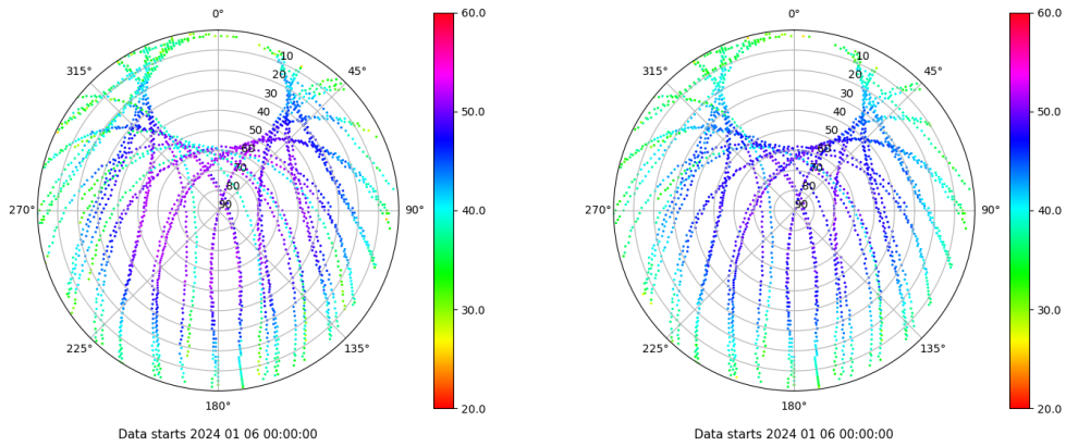
Skyplot for station VIGO. Signal to Noise S1C Data file VIGO00ESP_R_2024006.xtr Skyplot for station VIGO. Signal to Noise S2C Data file VIGO00ESP_R_2024006.xtr
