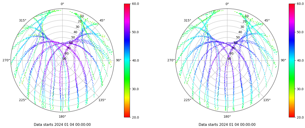
Skyplot for station VIGO. Signal to Noise S1C Data file VIGO00ESP_R_2024004.xtr Skyplot for station VIGO. Signal to Noise S2C Data file VIGO00ESP_R_2024004.xtr
