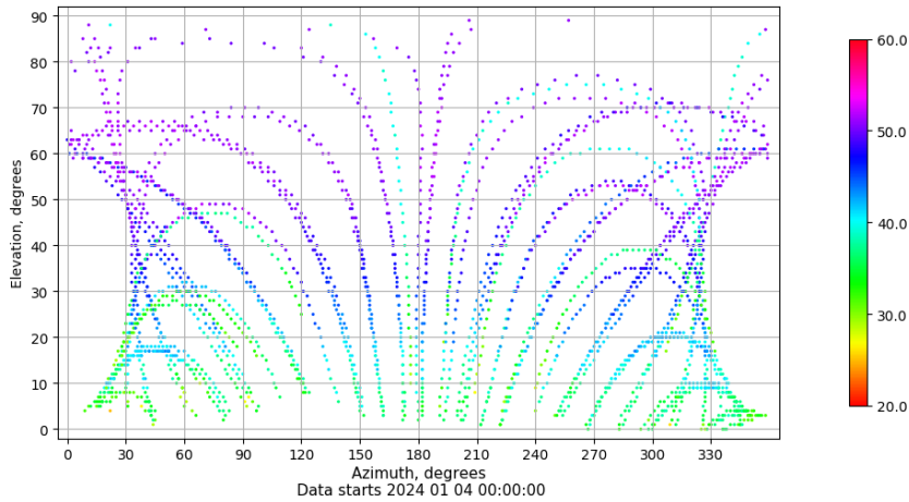
Azimuth-elevation plot for station VIGO. Signal to Noise S1C Data file VIGO00ESP_R_2024004.xtr
