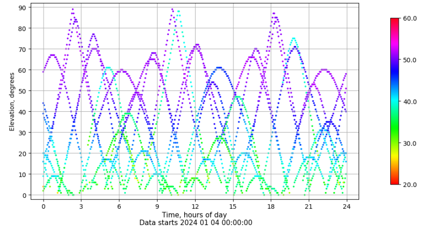
Time-elevation plot for station VIGO. Signal to Noise S1C Data file VIGO00ESP_R_2024004.xtr
