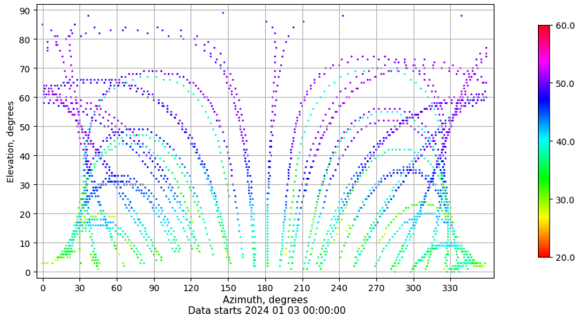
Azimuth-elevation plot for station VIGO. Signal to Noise S1C Data file VIGO00ESP_R_2024003.xtr
