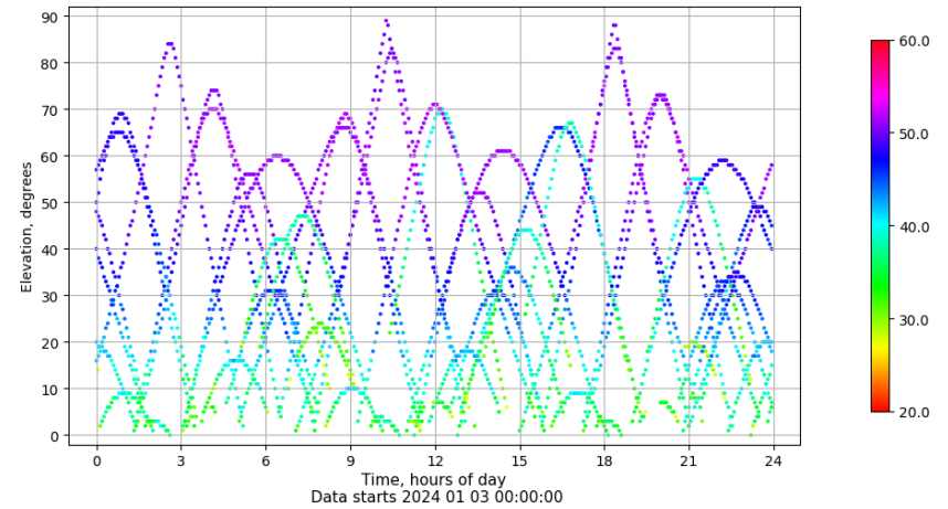
Time-elevation plot for station VIGO. Signal to Noise S1C Data file VIGO00ESP_R_2024003.xtr
