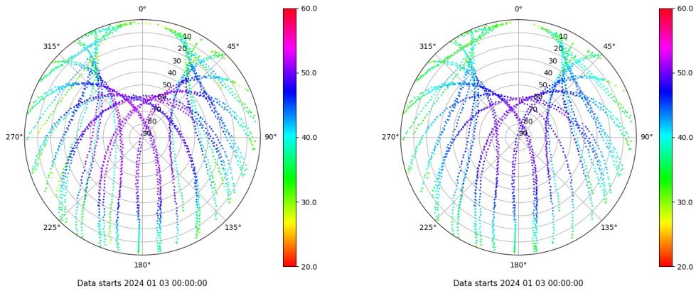
Skyplot for station VIGO. Signal to Noise S1C Data file VIGO00ESP_R_2024003.xtr Skyplot for station VIGO. Signal to Noise S2C Data file VIGO00ESP_R_2024003.xtr
