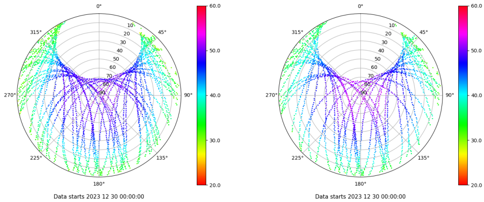
Skyplot for station VIGO. Signal to Noise S1C Data file VIGO00ESP_R_2023364.xtr Skyplot for station VIGO. Signal to Noise S2X Data file VIGO00ESP_R_2023364.xtr
