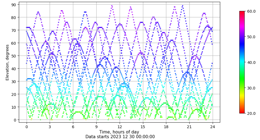
Time-elevation plot for station VIGO. Signal to Noise S1C Data file VIGO00ESP_R_2023364.xtr
