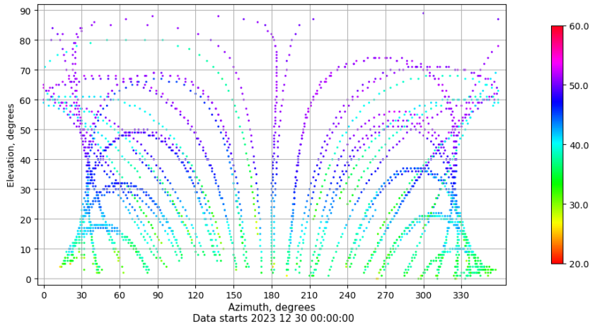
Azimuth-elevation plot for station VIGO. Signal to Noise S1C Data file VIGO00ESP_R_2023364.xtr
