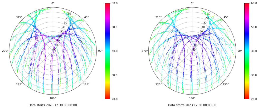
Skyplot for station VIGO. Signal to Noise S1C Data file VIGO00ESP_R_2023364.xtr Skyplot for station VIGO. Signal to Noise S2C Data file VIGO00ESP_R_2023364.xtr
