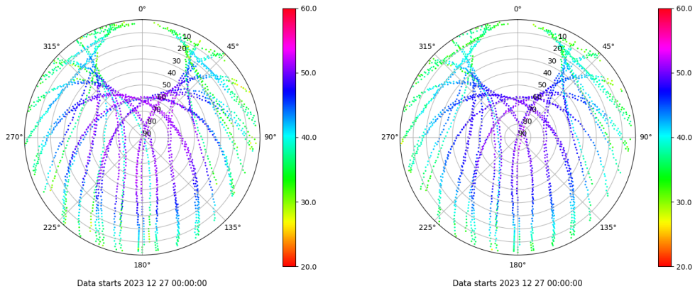
Skyplot for station VIGO. Signal to Noise S1C Data file VIGO00ESP_R_2023361.xtr Skyplot for station VIGO. Signal to Noise S2C Data file VIGO00ESP_R_2023361.xtr
