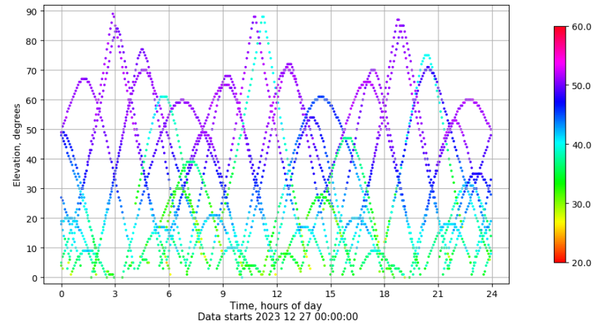
Time-elevation plot for station VIGO. Signal to Noise S1C Data file VIGO00ESP_R_2023361.xtr
