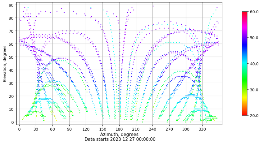
Azimuth-elevation plot for station VIGO. Signal to Noise S1C Data file VIGO00ESP_R_2023361.xtr
