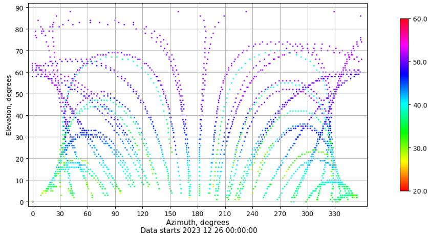
Azimuth-elevation plot for station VIGO. Signal to Noise S1C Data file VIGO00ESP_R_2023360.xtr
