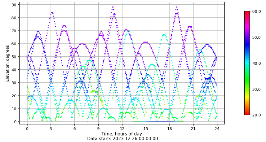
Time-elevation plot for station VIGO. Signal to Noise S1C Data file VIGO00ESP_R_2023360.xtr
