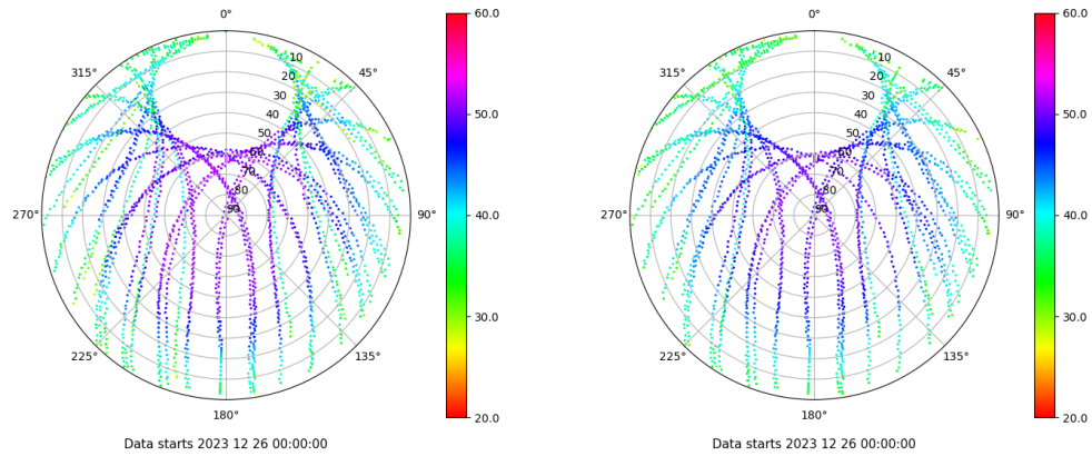
Skyplot for station VIGO. Signal to Noise S1C Data file VIGO00ESP_R_2023360.xtr Skyplot for station VIGO. Signal to Noise S2C Data file VIGO00ESP_R_2023360.xtr
