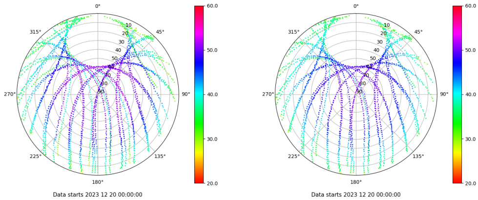
Skyplot for station VIGO. Signal to Noise S1C Data file VIGO00ESP_R_2023354.xtr Skyplot for station VIGO. Signal to Noise S2C Data file VIGO00ESP_R_2023354.xtr
