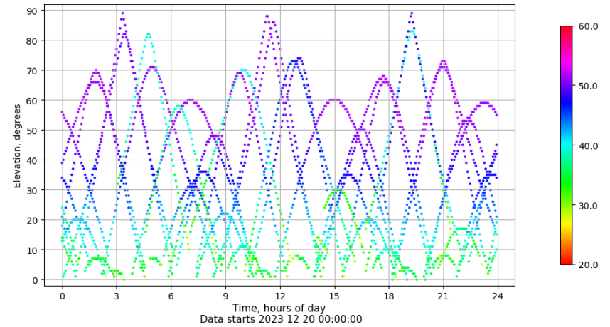
Time-elevation plot for station VIGO. Signal to Noise S1C Data file VIGO00ESP_R_2023354.xtr
