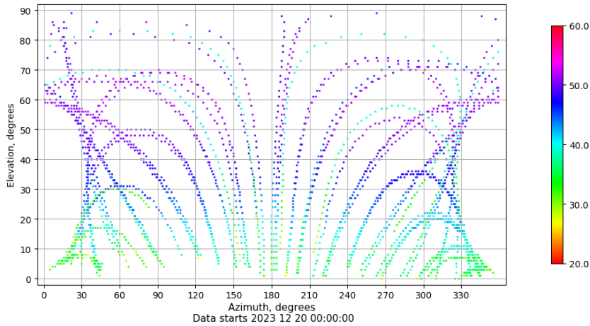
Azimuth-elevation plot for station VIGO. Signal to Noise S1C Data file VIGO00ESP_R_2023354.xtr
