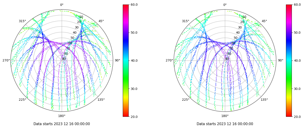
Skyplot for station VIGO. Signal to Noise S1C Data file VIGO00ESP_R_2023350.xtr Skyplot for station VIGO. Signal to Noise S2C Data file VIGO00ESP_R_2023350.xtr
