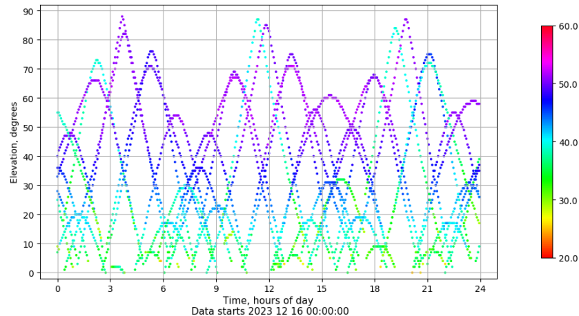
Time-elevation plot for station VIGO. Signal to Noise S1C Data file VIGO00ESP_R_2023350.xtr
