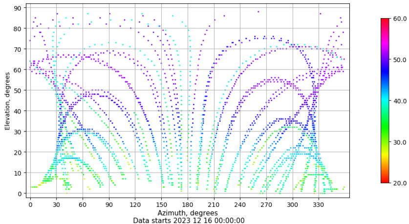
Azimuth-elevation plot for station VIGO. Signal to Noise S1C Data file VIGO00ESP_R_2023350.xtr
