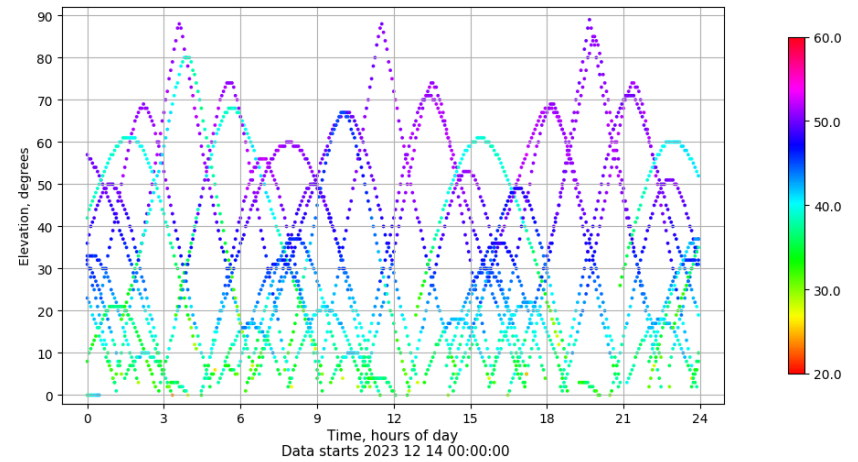
Time-elevation plot for station VIGO. Signal to Noise S1C Data file VIGO00ESP_R_2023348.xtr
