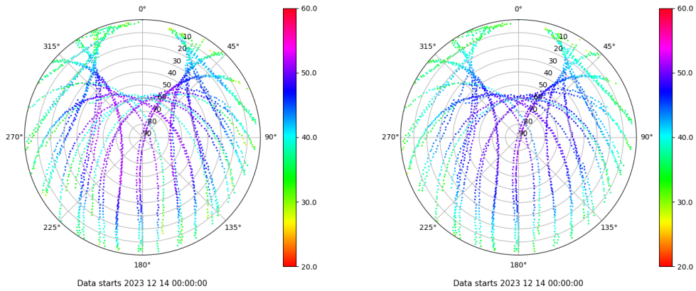
Skyplot for station VIGO. Signal to Noise S1C Data file VIGO00ESP_R_2023348.xtr Skyplot for station VIGO. Signal to Noise S2C Data file VIGO00ESP_R_2023348.xtr
