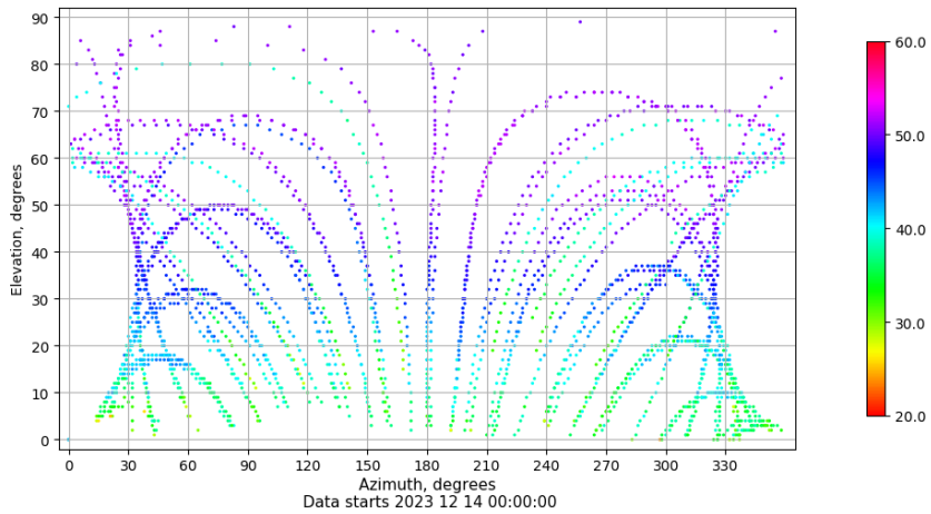
Azimuth-elevation plot for station VIGO. Signal to Noise S1C Data file VIGO00ESP_R_2023348.xtr
