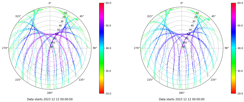
Skyplot for station VIGO. Signal to Noise S1C Data file VIGO00ESP_R_2023346.xtr Skyplot for station VIGO. Signal to Noise S2C Data file VIGO00ESP_R_2023346.xtr
