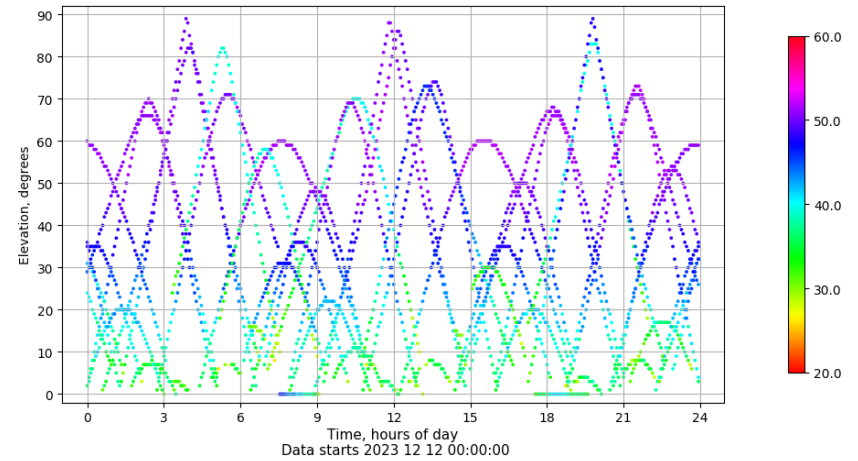
Time-elevation plot for station VIGO. Signal to Noise S1C Data file VIGO00ESP_R_2023346.xtr
