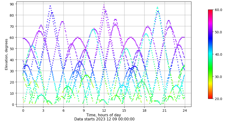
Time-elevation plot for station VIGO. Signal to Noise S1C Data file VIGO00ESP_R_2023343.xtr
