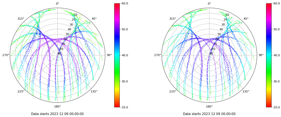
Skyplot for station VIGO. Signal to Noise S1C Data file VIGO00ESP_R_2023343.xtr Skyplot for station VIGO. Signal to Noise S2C Data file VIGO00ESP_R_2023343.xtr
