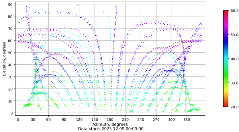
Azimuth-elevation plot for station VIGO. Signal to Noise S1C Data file VIGO00ESP_R_2023343.xtr
