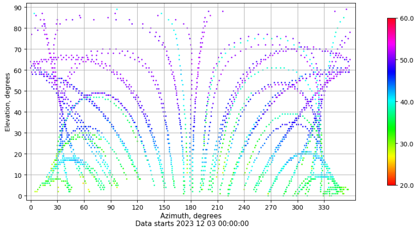
Azimuth-elevation plot for station VIGO. Signal to Noise S1C Data file VIGO00ESP_R_2023337.xtr
