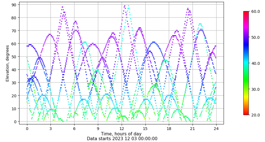
Time-elevation plot for station VIGO. Signal to Noise S1C Data file VIGO00ESP_R_2023337.xtr
