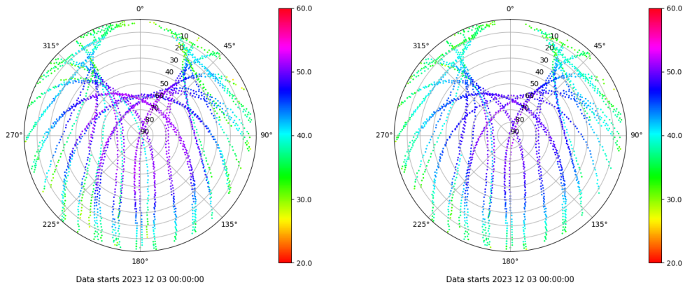
Skyplot for station VIGO. Signal to Noise S1C Data file VIGO00ESP_R_2023337.xtr Skyplot for station VIGO. Signal to Noise S2C Data file VIGO00ESP_R_2023337.xtr
