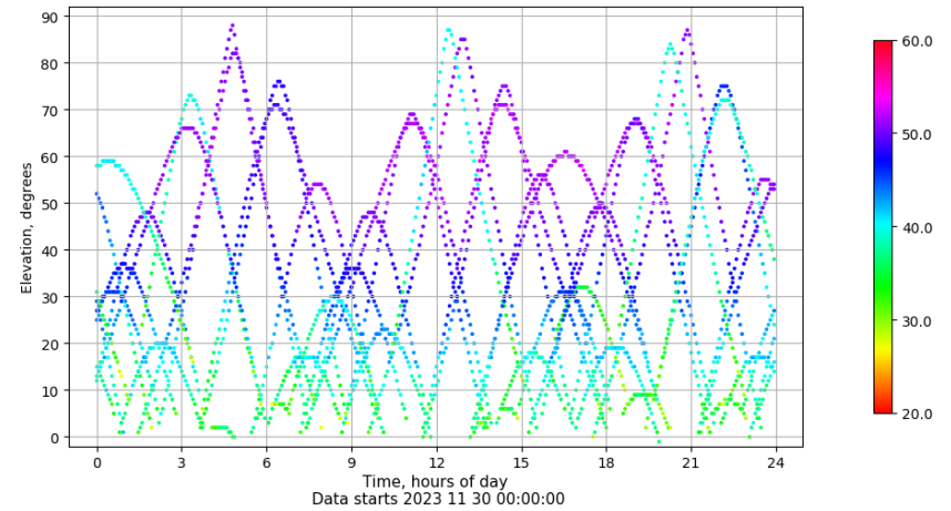
Time-elevation plot for station VIGO. Signal to Noise S1C Data file VIGO00ESP_R_2023334.xtr
