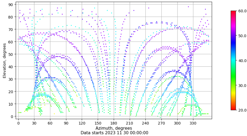
Azimuth-elevation plot for station VIGO. Signal to Noise S1C Data file VIGO00ESP_R_2023334.xtr
