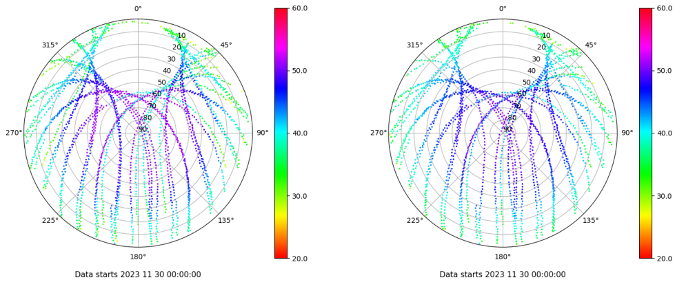
Skyplot for station VIGO. Signal to Noise S1C Data file VIGO00ESP_R_2023334.xtr Skyplot for station VIGO. Signal to Noise S2C Data file VIGO00ESP_R_2023334.xtr
